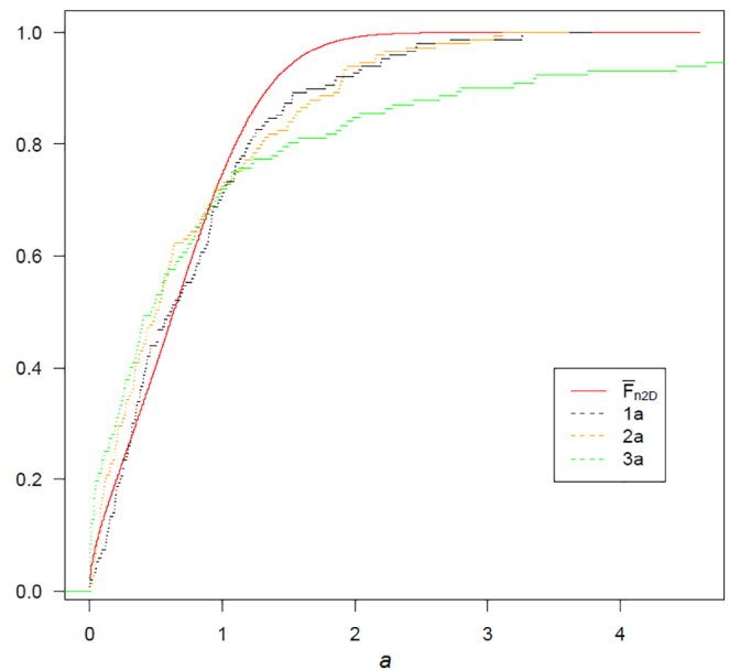
FIGURE 20 Cumulative distribution function comparison of the cells area of the schemes of plane sections of alumina ceramics (Figure 19 1a black line, 2a yellow line, 3a green line) and of the two-dimension sectional Poisson-Voronoi cells area (red line) [Colour figure can be viewed at wileyonlinelibrary.com ]
