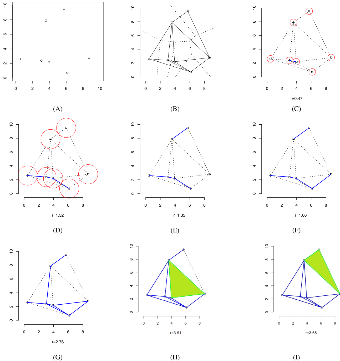
FIGURE 4 (A) Set of points X , (B) Voronoi diagram (dashed) and Delaunay triangulation (solid), (C) Circles with radius 0.47 around the points of X ; the Alpha complex \alpha_r(X) consists of the individual points of X and the one edge corresponding to the two touching circles, (D) Alpha complex for r = 1.32 , (E) Alpha complex, r = 1.35 , (F) Alpha complex, r = 1.66 , (G) Alpha complex, r = 2.76 , (H) Alpha complex, r = 3.61 , and (I) Alpha complex, r = 3.68 [Colour figure can be viewed at wileyonlinelibrary.com ]
