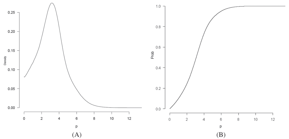
FIGURE 2 (A) Boundary corrected Kernel density estimate (Epanechnikov kernel, linear combination correction, h = 0.1^{12} ) and (B) empirical cumulative distribution function of the perimeter of 36 480 600 two-dimension sectional cells, \lambda = 1
