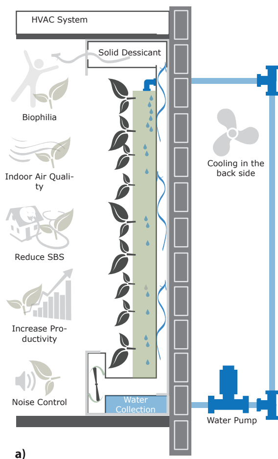
Figure 3. Prototype. a) Diagram of the LWS Design, b) LWS scaled Prototype and Data logger location, c) Section. (Armijos Moya, 2016)
