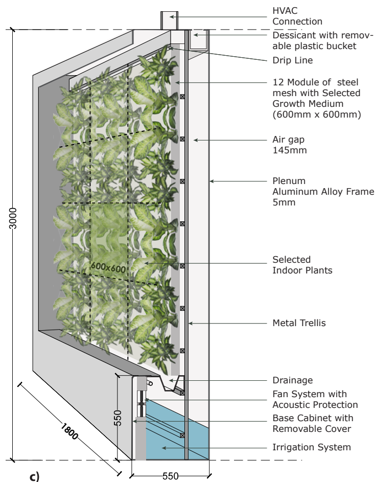
Figure 3. Prototype. a) Diagram of the LWS Design, b) LWS scaled Prototype and Data logger location, c) Section. (Armijos Moya, 2016)
