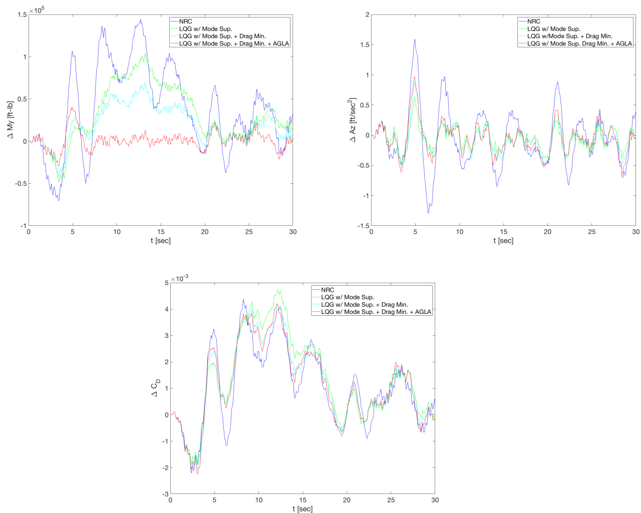
Figure 9. Performance Response to Multi-Objective Flight Control with Mode Suppression, Drag Minimization and Active Gust Load Alleviation
