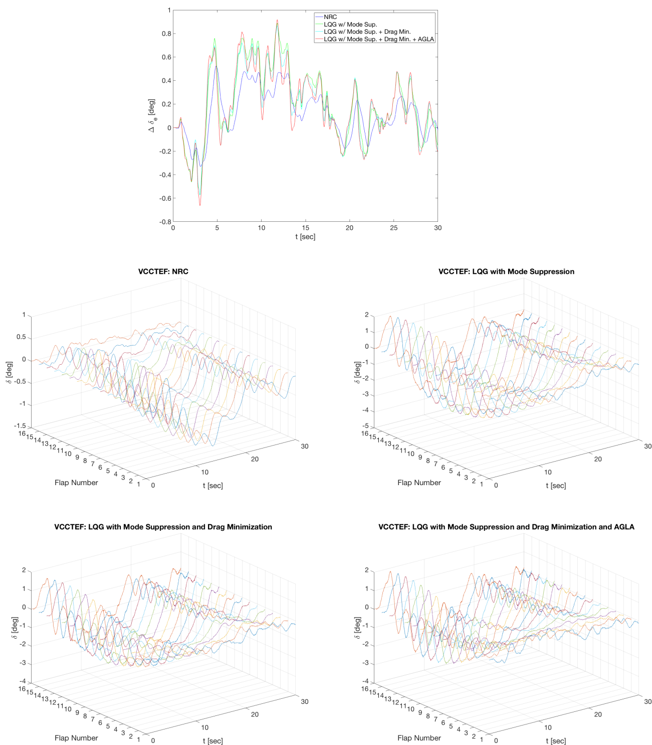
Figure 8. Control Surface Deflections for Multi-Objective Flight Control with Mode Suppression and Drag Minimization
