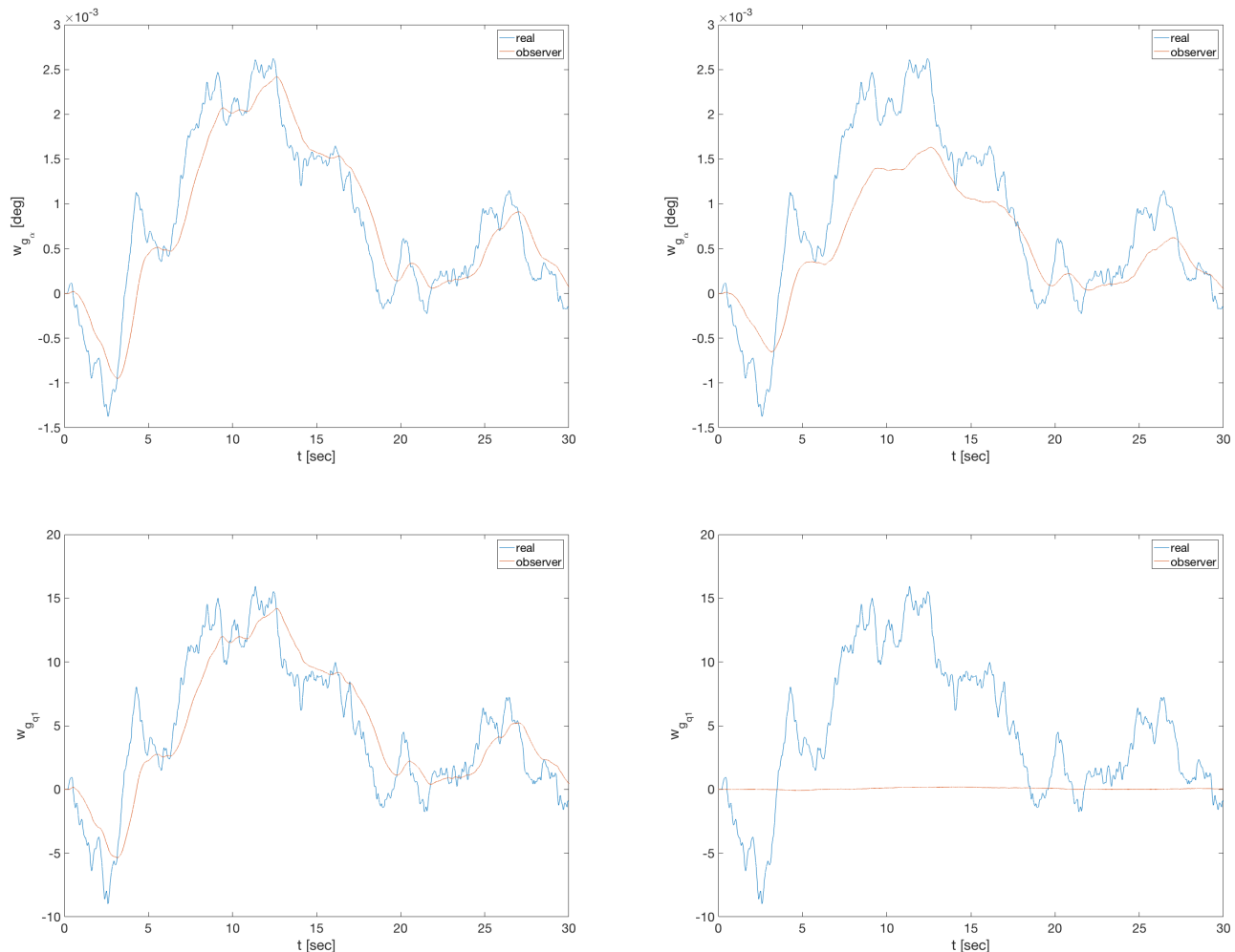
Figure 10. ESO Disturbance Estimation
