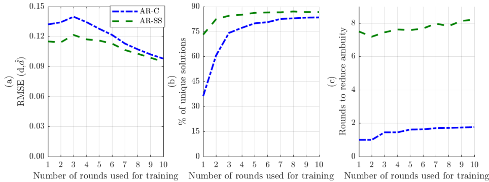
Figure 5.3: Reducing ambiguity: (a) Precision; (b) Unique solutions; (c) Number of interactions made for reducing ambiguity.
