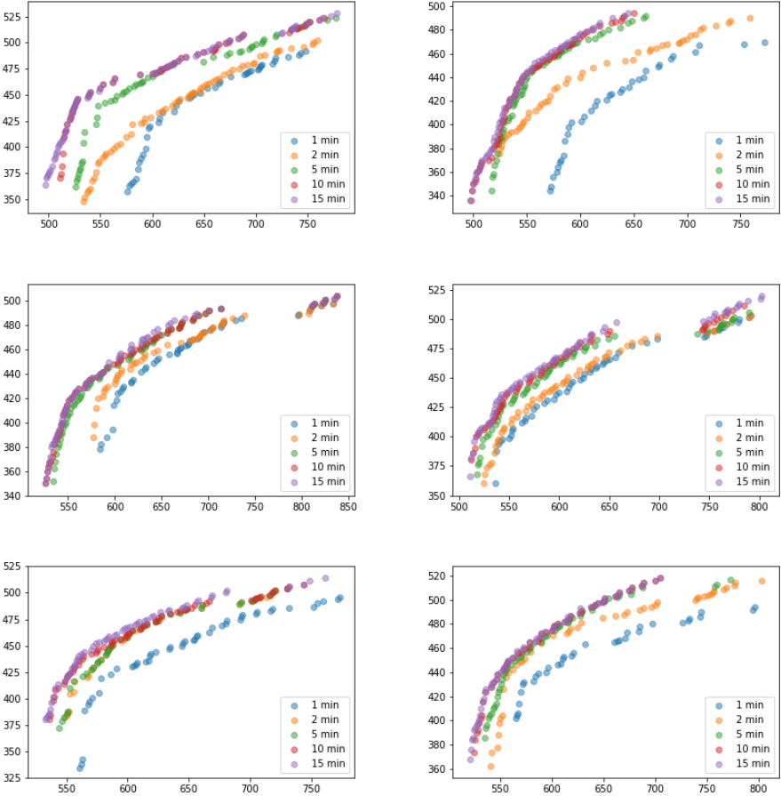
Figure 4.B.3: Estimated Pareto frontiers via the metaheuristic at different time instants for instances of size 100 students.
