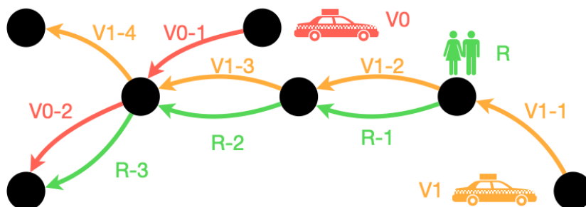
Figure 3.1: Example of moves. Colours refer to who is travelling that arc (red for vehicle V_0 , yellow for vehicle V_1 and green for request R ). The text next to each arc indicates who is travelling that arc and at which move.
