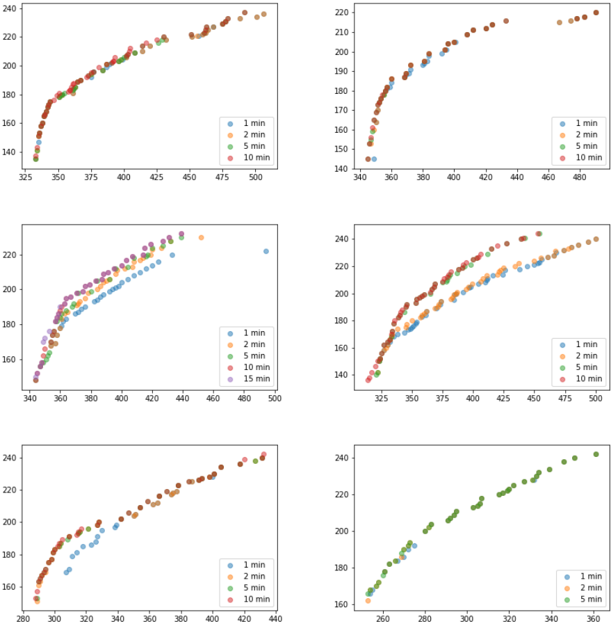
Figure 4.B.1: Estimated Pareto frontiers via the metaheuristic at different time instants for instances of size 50 students.
