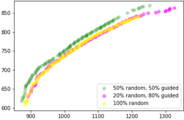
Figure 4.B.4: Different estimated Pareto frontiers depending on the probability of selecting a guided search. On the x-axis, the routing cost; on the y-axis, the quality of service.
