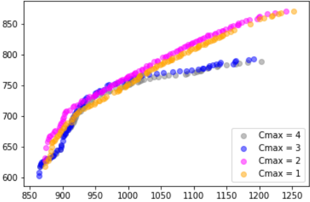
Figure 4.B.5: Estimated Pareto frontiers for different C_{max} values. On the x-axis, the routing cost; on the y-axis, the quality of service.
