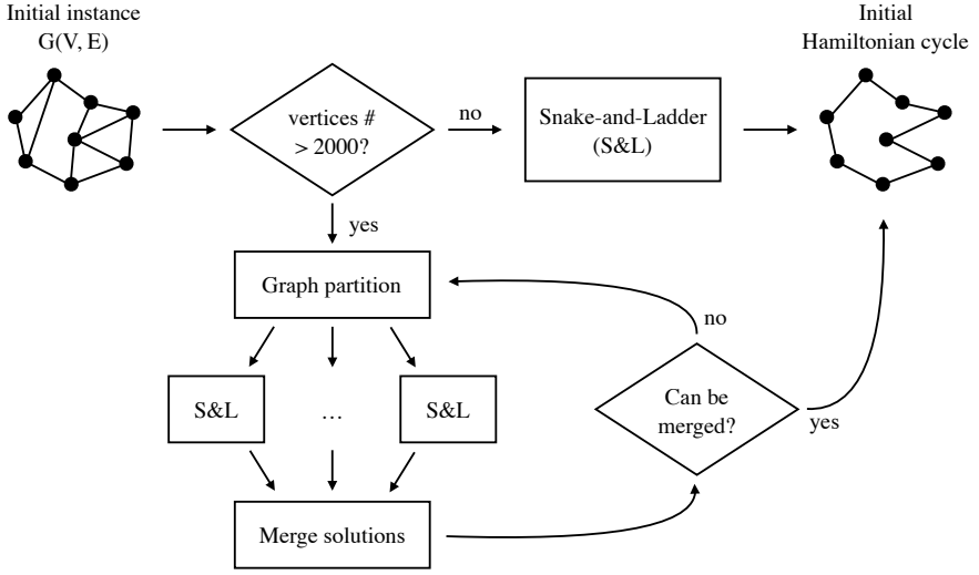
Figure 2.2: Flowchart of the process to generate the initial solution.
