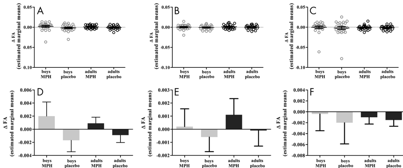
Figure 3: A–F, Graphs show results of region of interest analysis. A–C, Scatterplots of changes in raw fractional anisotropy (FA) values from baseline to after treatment in, A, whole-brain white matter, B, anterior thalamic radiation, and, C, splenium. D–F, Box-and-whisker plots show estimated marginal means and standard errors for change in FA values from baseline to after treatment in, D, whole-brain white matter, E, anterior thalamic radiation, and, F, splenium. Error bars = standard errors of the mean. MPH = methylphenidate.
