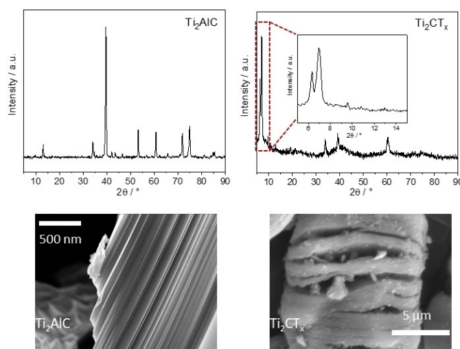
Figure 1. XRD patterns and SEM images of Ti_2AlC MAX phase and Ti_2CT_x MXene.
