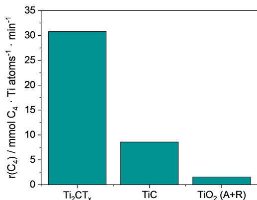
Figure 2. C_4 olefin formation rate of the studied catalysts after 0.5 h under reaction at 500 °C and \text{O}_2/\text{butane} = 1:1 . A + R denotes anatase + rutile titania.
