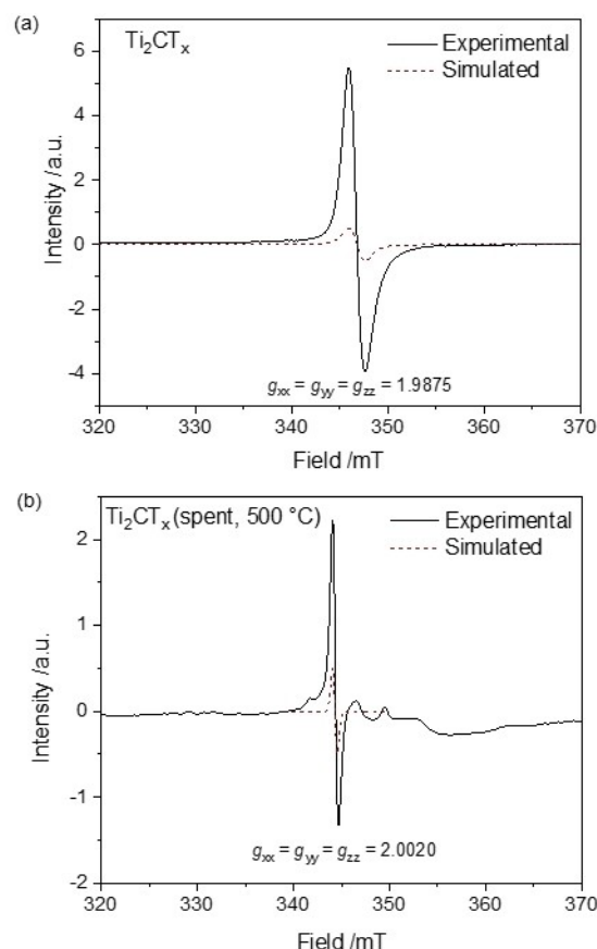
Figure 3. Experimental (measured at 10 K) and simulated EPR spectra of (a) \text{Ti}_2\text{CT}_x MXene fresh and (b) after the stability test at 500 °C. Experimental parameters; microwave frequency (a) 9.648388 GHz and (b) 9.647805, power 0.6325 mW, modulation amplitude 4.000 G.
