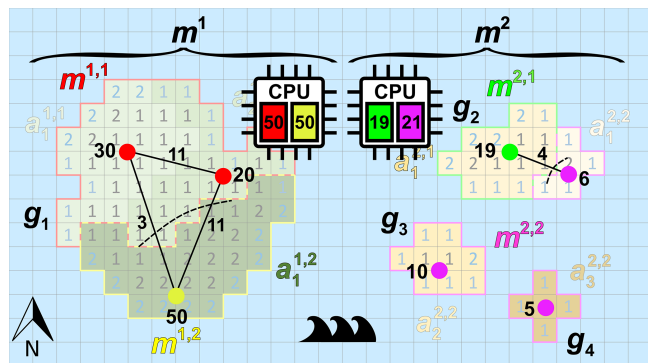
Figure 8. Example of area-based graph partitioning corresponding to the example of Fig. 3, where the work for each submodel is uniquely assigned to a core of a dual-core CPU.
