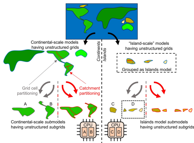
Figure 1. General concept of defining GLOBGM as a set of independent (larger) continental-scale groundwater models (left-hand side) and (smaller) island-scale groundwater models as a remaining model (right-hand side). All of these models have independent unstructured grids that are partitioned by (a) straightforwardly assigning grid cells (grid cell partitioning; gray arrows) or (b) assigning catchments (catchment partitioning; red arrows). The resulting subgrids define the computational cells for the submodels that are uniquely assigned to a processor core/MPI process. In this figure, this is illustrated by assigning submodels “A” and “B” to one dual-core CPU and submodels “C” and “D” to another.
