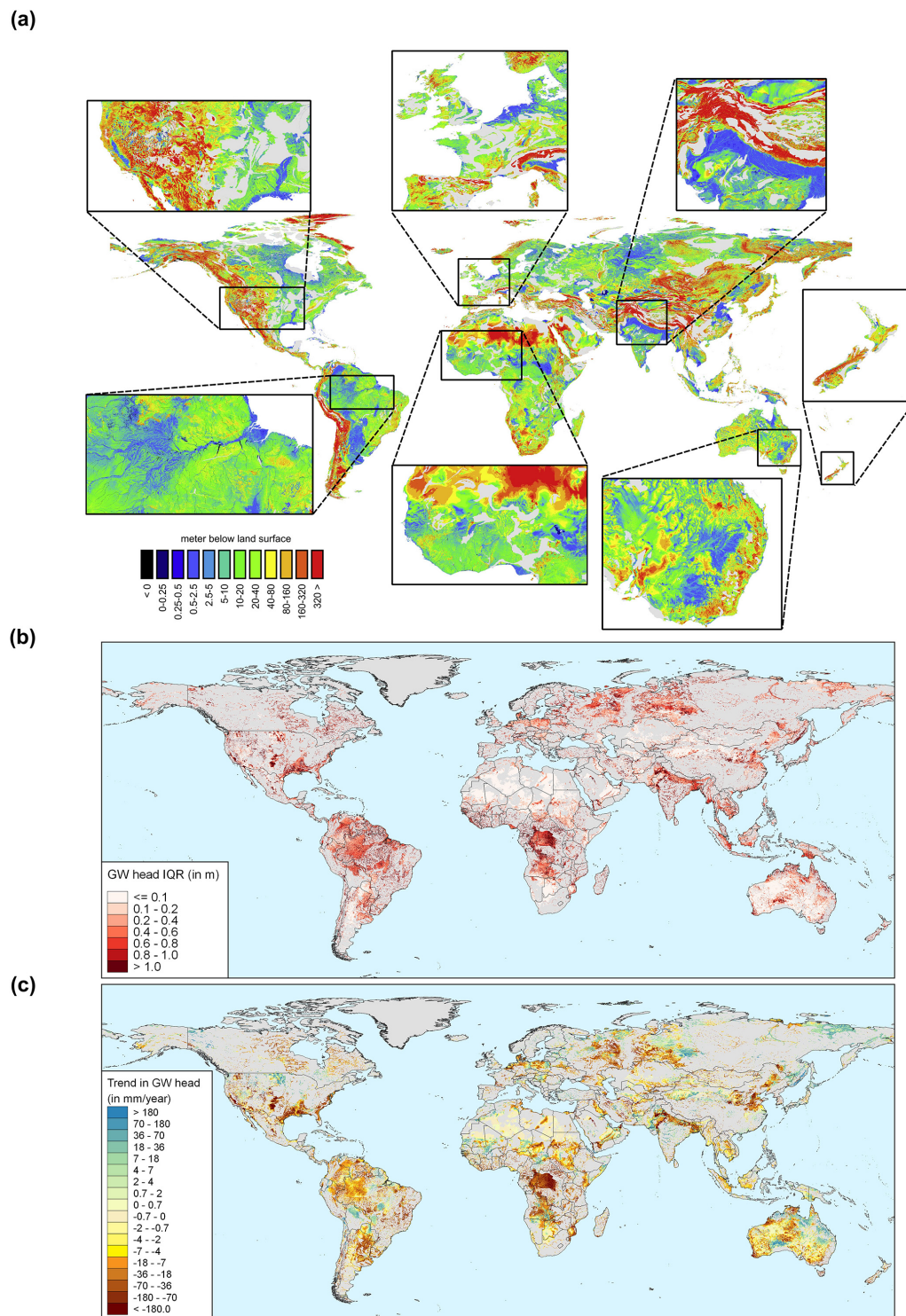
Figure 16. Example outputs of GLOBGM. (a) Steady-state water table depth with detailed zoomed-in insets. (b) Water table amplitude for 2003–2015, as represented by the interquartile range (IQR). (c) Hydraulic head trends for 2003–2015 for the aquifer (lower model layer). In all panels, a mask is applied for karst areas; in the lower panels of (b) and (c), an additional mask is applied for mountain ranges.
