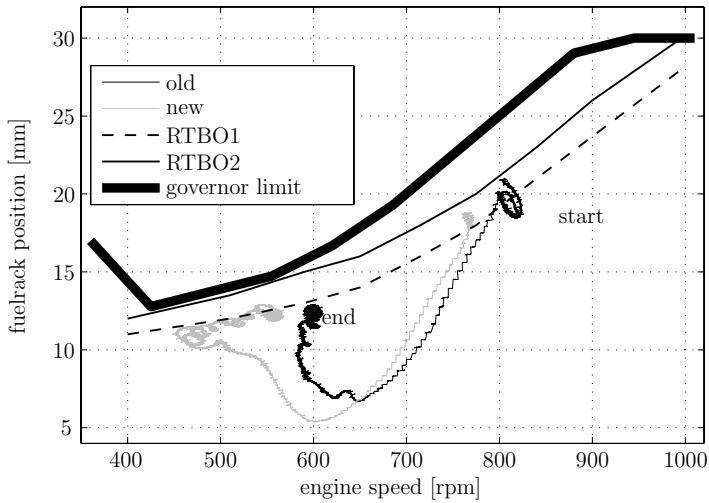
Figure 9.27: Engine diagram
