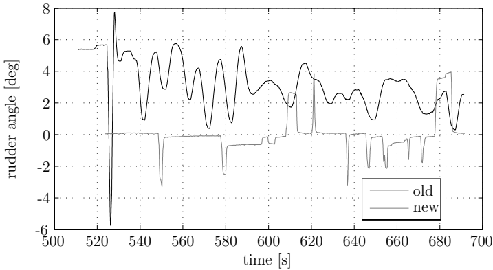
Figure 9.3: Rudder
