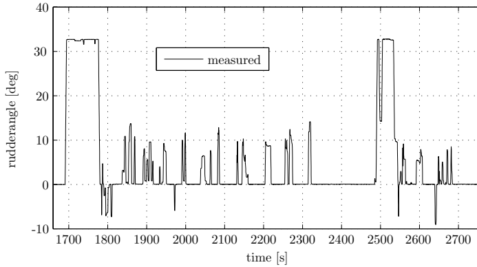
Figure 5.12: Disturbing input during validation experiment: rudder angle
