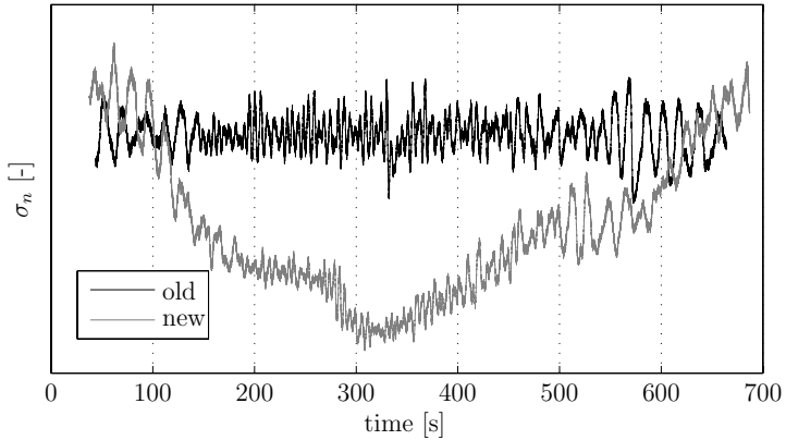
Figure 9.64: Cavitation number
