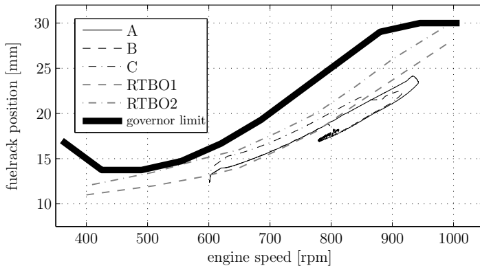
Figure 7.24: Prediction of behaviour in the engine diagram
