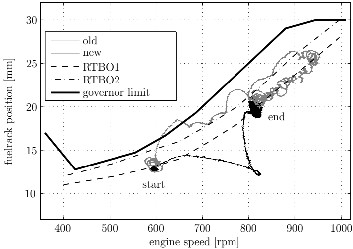
Figure 9.8: Engine diagram
