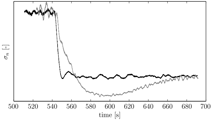
Figure 9.14: Cavitation number
