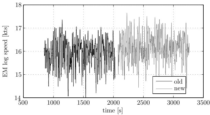
Figure 9.49: Ship speed
