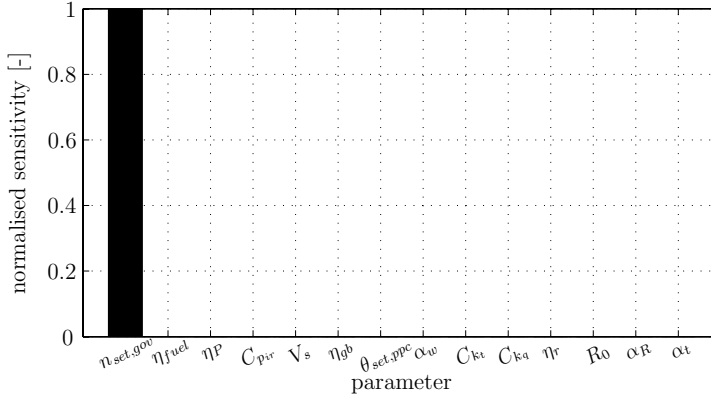
Figure 5.24: Absolute normalised sensitivity of shaft speed n in operating point II
