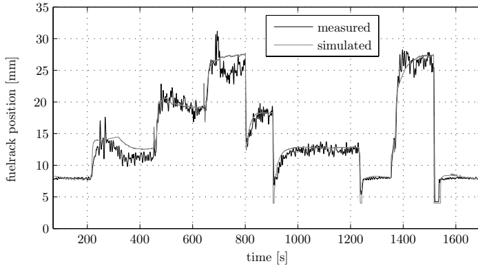
Figure 4.25: Total model output: fuelrack position X
