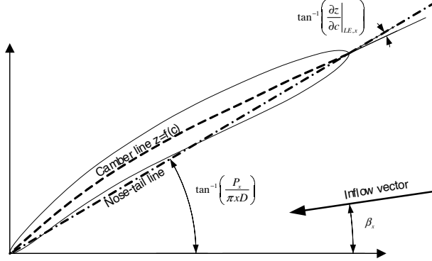
Figure 7.6: Propeller section inflow definitions
