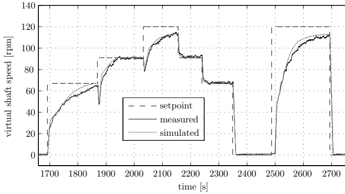
Figure 5.11: Validation input: the command and realised virtual shaft speed
