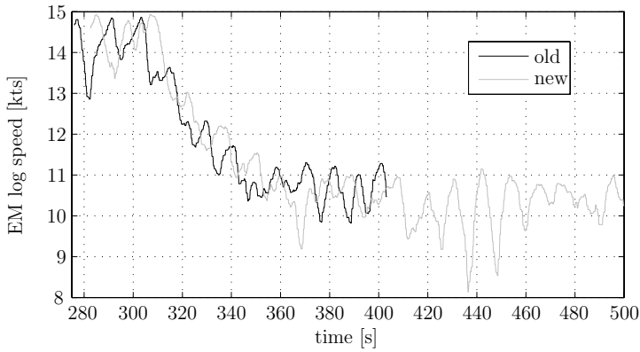
Figure 9.29: Ship speed
