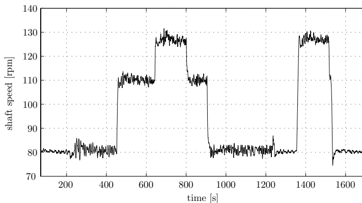
Figure 4.8: Enforced input of the propeller model: shaft speed n
