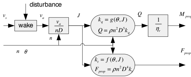
Figure 2.5: Hydrodynamic Propeller blockdiagram
