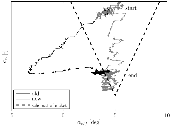
Figure 9.15: \alpha bucket
