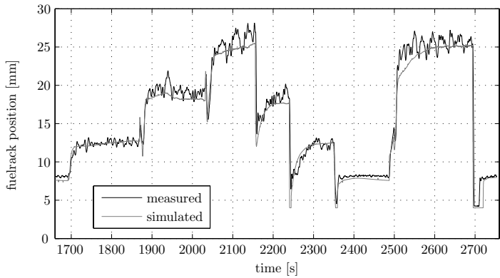
Figure 5.17: Validation: fuelrack position
