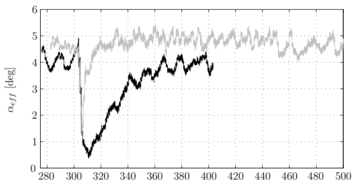
Figure 9.32: Estimated effective angle of attack
