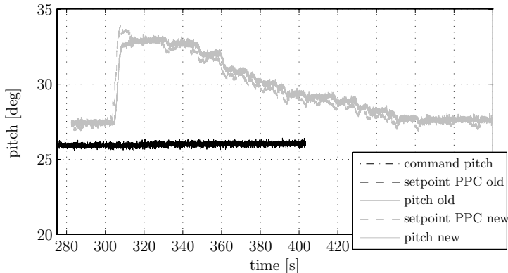
Figure 9.25: Low level pitch setpoint and pitch
