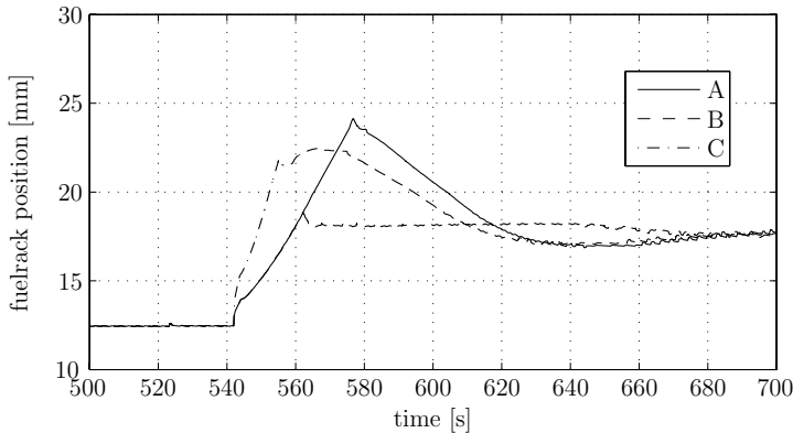
Figure 7.23: Simulated fuelrack
