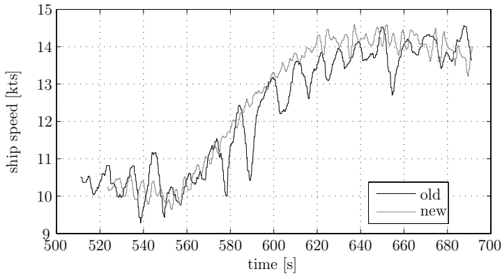
Figure 9.10: Ship speed
