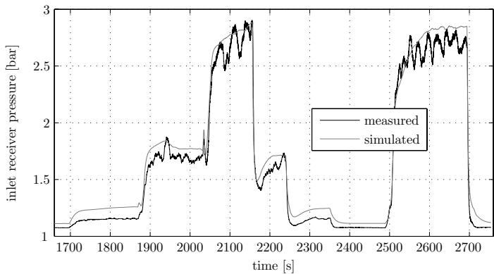
Figure 5.18: Validation: inlet receiver pressure
