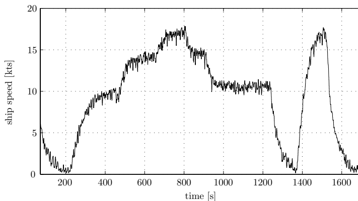
Figure 4.9: Enforced input of the propeller model: ship speed v_s
