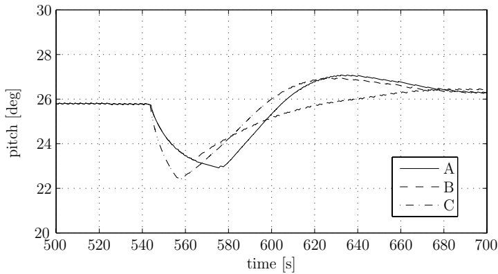
Figure 7.19: Simulated pitch
