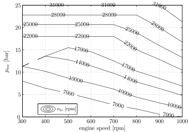
Figure A.3: Engine lookup table 3
