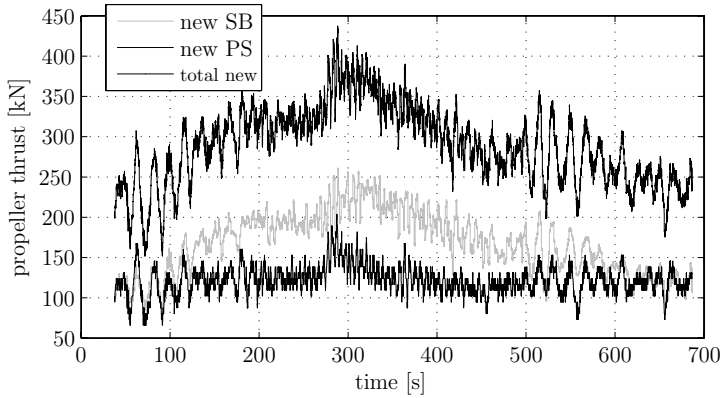
Figure 9.62: Thrust PCS+
