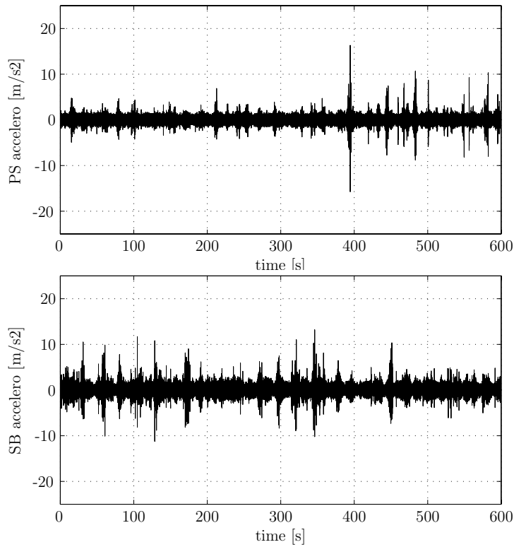
Figure 9.52: Acceleration sensor signals old PCS
