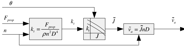
Figure 7.8: Advance velocity estimation process
