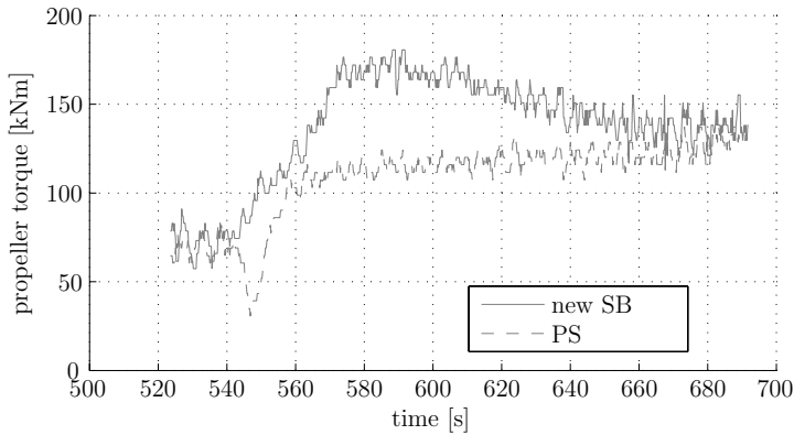
Figure 9.11: Propeller torque (port and starboard) for the old and the new PCS
