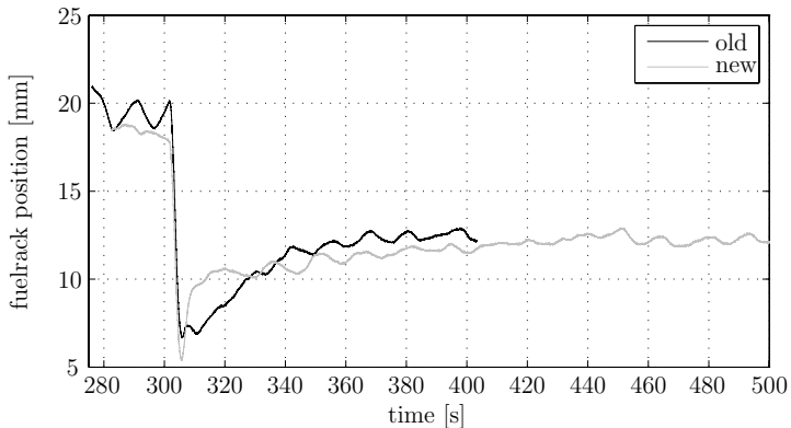
Figure 9.26: Fuelrack position
