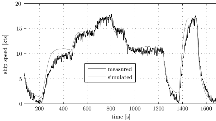
Figure 4.17: Output of the ship model: ship speed v_s
