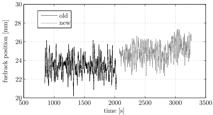
Figure 9.47: Fuelrack position
