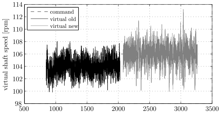
Figure 9.43: Command
