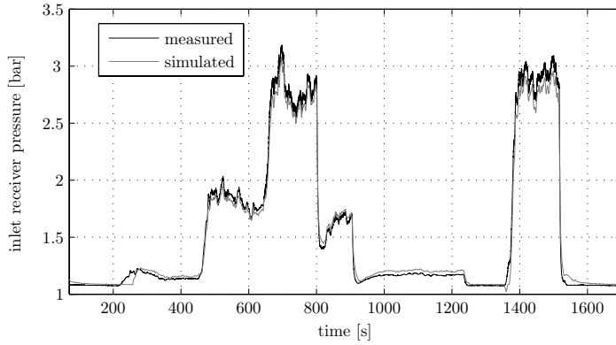
Figure 4.6: Output of the calibrated engine model: inlet receiver pressure p_{ir}
