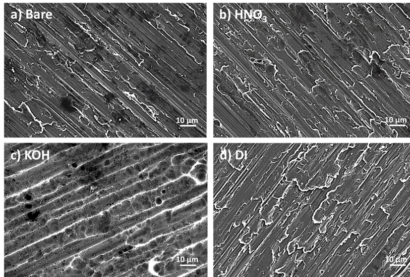
Fig. 4. SEM images of (a) bare Al (800 grit) and Al (800 grit) pre-treated with (b) HNO 3 , (c) KOH and with (d) boiling DI water. The SEM images were taken in secondary electron imaging (SEI) mode.
