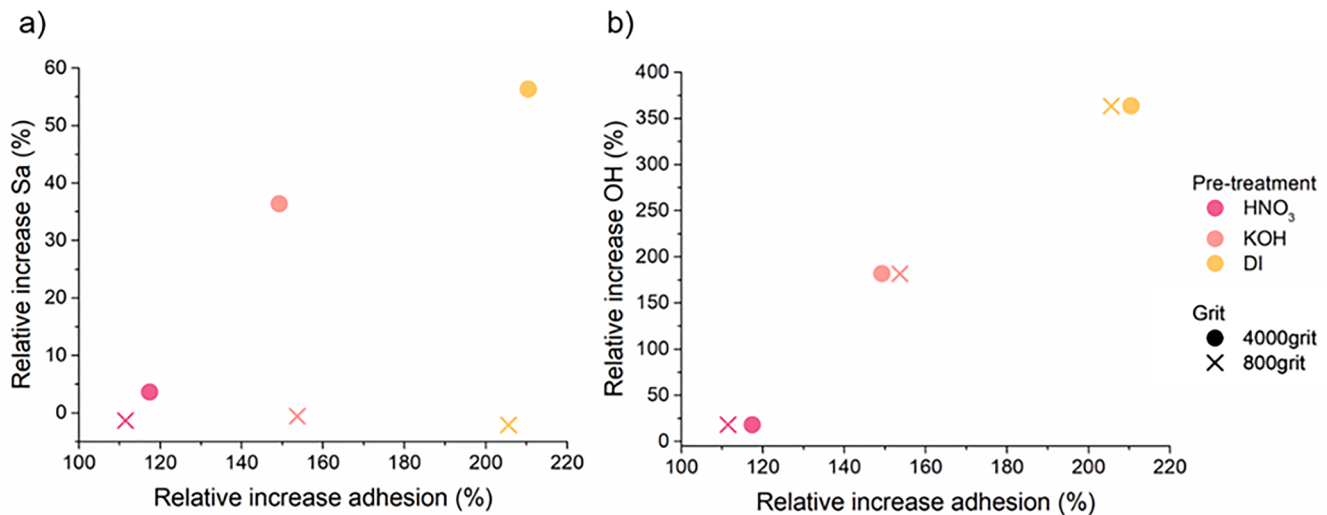
Fig. 10. Relative increases of (a) S_a versus adhesion and (b) OH versus adhesion.
