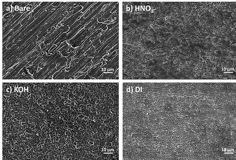
Fig. 3. SEM images of (a) bare Al (4000 grit) and Al (4000 grit) pre-treated with (b) HNO 3 , (c) KOH and with (d) boiling DI water. The SEM images were taken in secondary electron imaging (SEI) mode.
