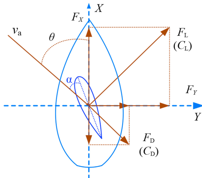
Fig. 3. Diagram of the wing force analysis.
