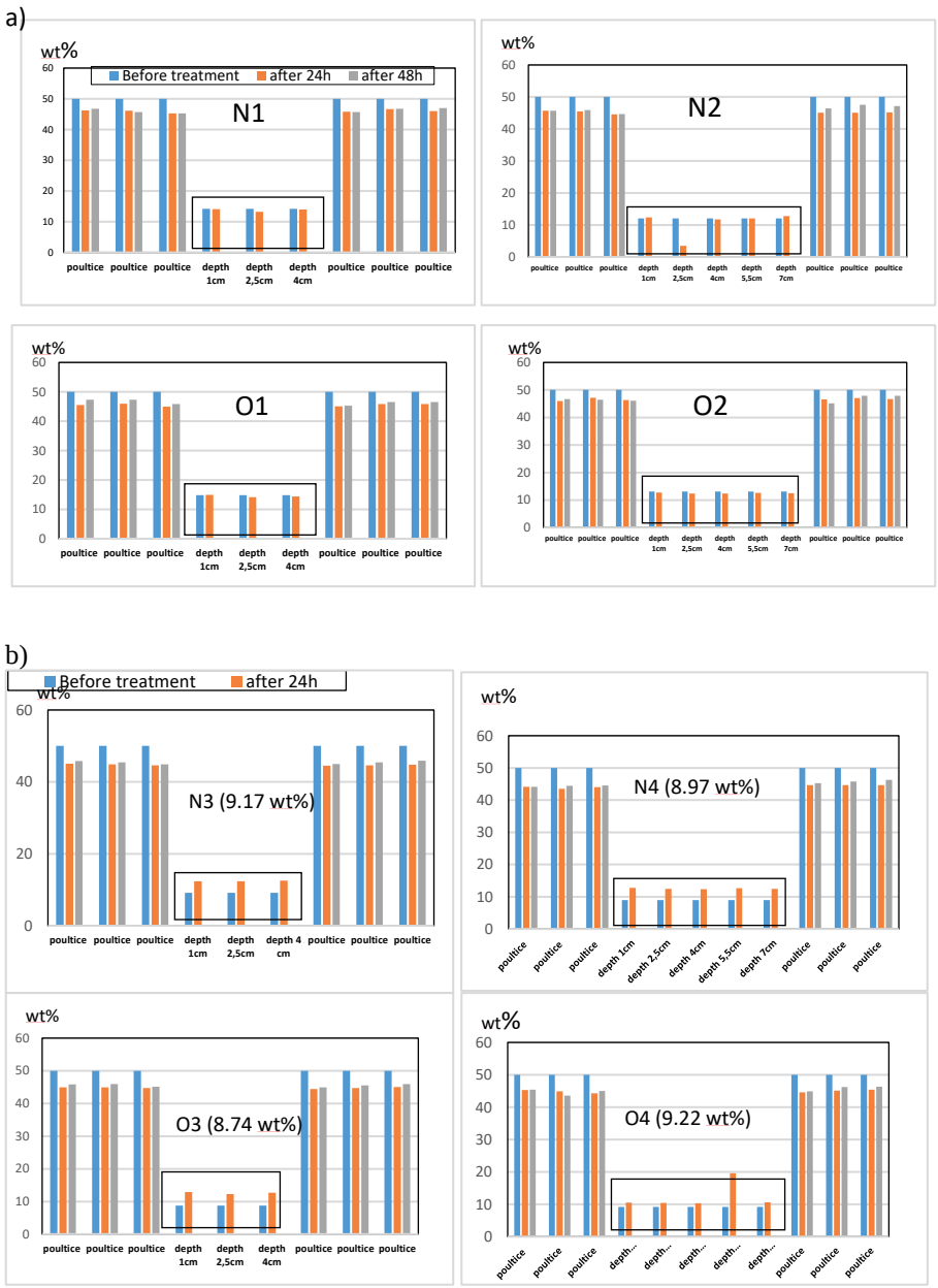
Figure 5: Water content differences both in bricks O and N (at different depths) and poultices in completely saturated and partially saturated samples (the anode is placed at the left and the cathode at the right).
