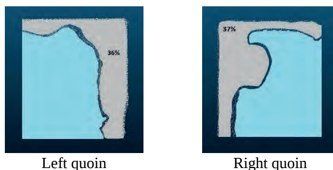
Figure 4: Quantification of matter loss in the tuffeau stonework supporting the arch. In blue: cross section at the most damaged stone course; in grey: outline of the reference stone course.
