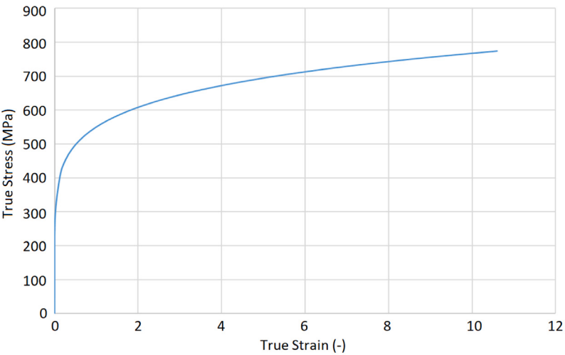
(a) Steel material model multi-linear
