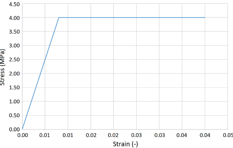
Fig. 6. Aluminium material model bi-linear.
