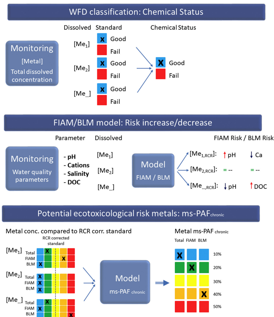
Fig. 1. Overview of three steps to take to translate monitoring data on the dissolved metal concentrations and local water quality towards a ms-PAF based ecotoxicological risk characterization for metals using either the dissolved metal concentration, a FIAM model corrected RCR_{FIAM} or a BLM corrected RCR_{BLM} . Step 1 shows the WFD classification of the chemical status based on dissolved metal concentrations. Step 2 uses the local water quality in combination with either the FIAM or the BLM model to indicate if there is an increase or decrease in the location specific metal risks based on local water quality parameters, indicated by an upward (higher risk) or downward (lower risk) arrow. In Step 3 the ms-PAF is calculated for all three methods, scoring the potential ecotoxicological impact on a scale of 0% to 50% potential mortality. In this example the dissolved metal based ms-PAF is 10%, not taking into account the local water quality parameters. The FIAM based ms-PAF is 20%, caused by a higher RCR_{FIAM} for metal 1. The RCR_{FIAM} for metal 1 is increased due to a locally lower PH as compared to standard water (see step 2). The BLM based ms-PAF is 40% due to an increased RCR_{BLM} for metal 3. This increase is caused by a deviation of the DOC concentration (lower) as compared to standard water (see step 2).
