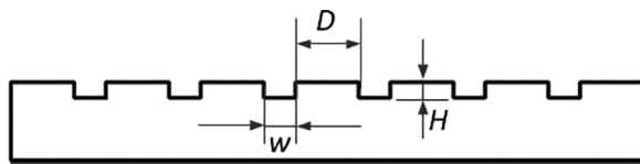
Figure 8. Geometrical model of a bionic groove surface (Han et al. 2012).
