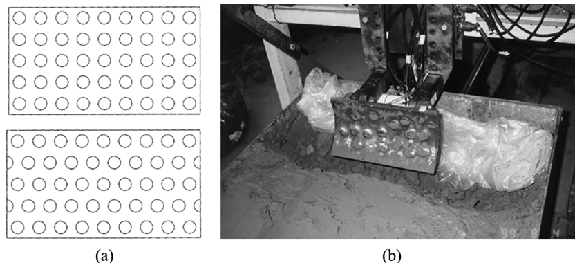
Figure 3. Application of convex domes on a bulldozing plate: (a) geometrical model (Ren et al. 1995) and (b) bionic model (Ren et al. 2002).
