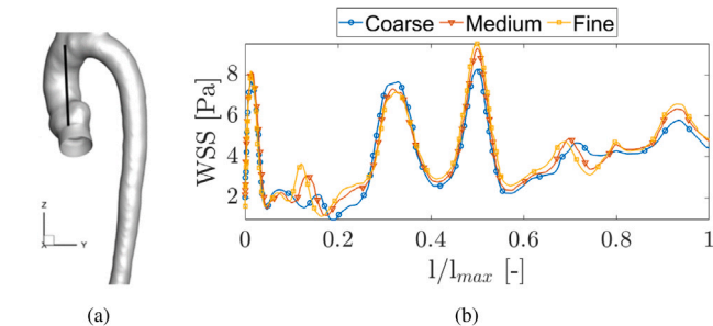
Fig. A.12. Extracted local Wall shear stress (WSS [Pa]) alongside the line visualized in (a) with normalized length l/l_{max} [-] where l_{max} is the total distance of the line, for the healthy control with lumen-only approximation, using coarse, medium, and fine mesh.
