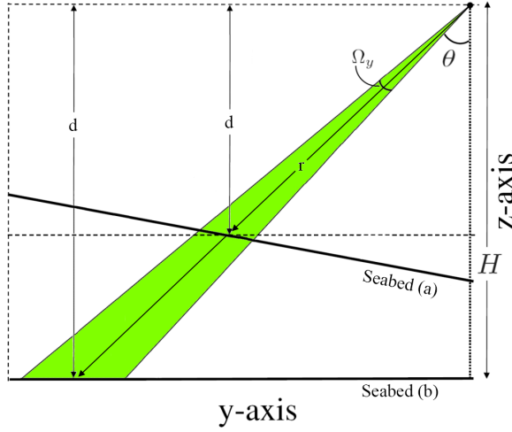
Figure 2.4: Cross-track cross section of an oblique beam of a multibeam echosounder for a sloping seabed (a) and a flat seabed (b). The range r from the sonar to the seabed, and the depth d are also shown (figure after [21] and [22]).
