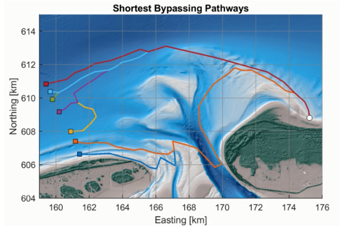
Figure 6. Shortest (dominant) bypassing pathways from 7 nodes offshore of Terschelling (the updrift side of the inlet) to a single point on the (downdrift) coast of Ameland.
