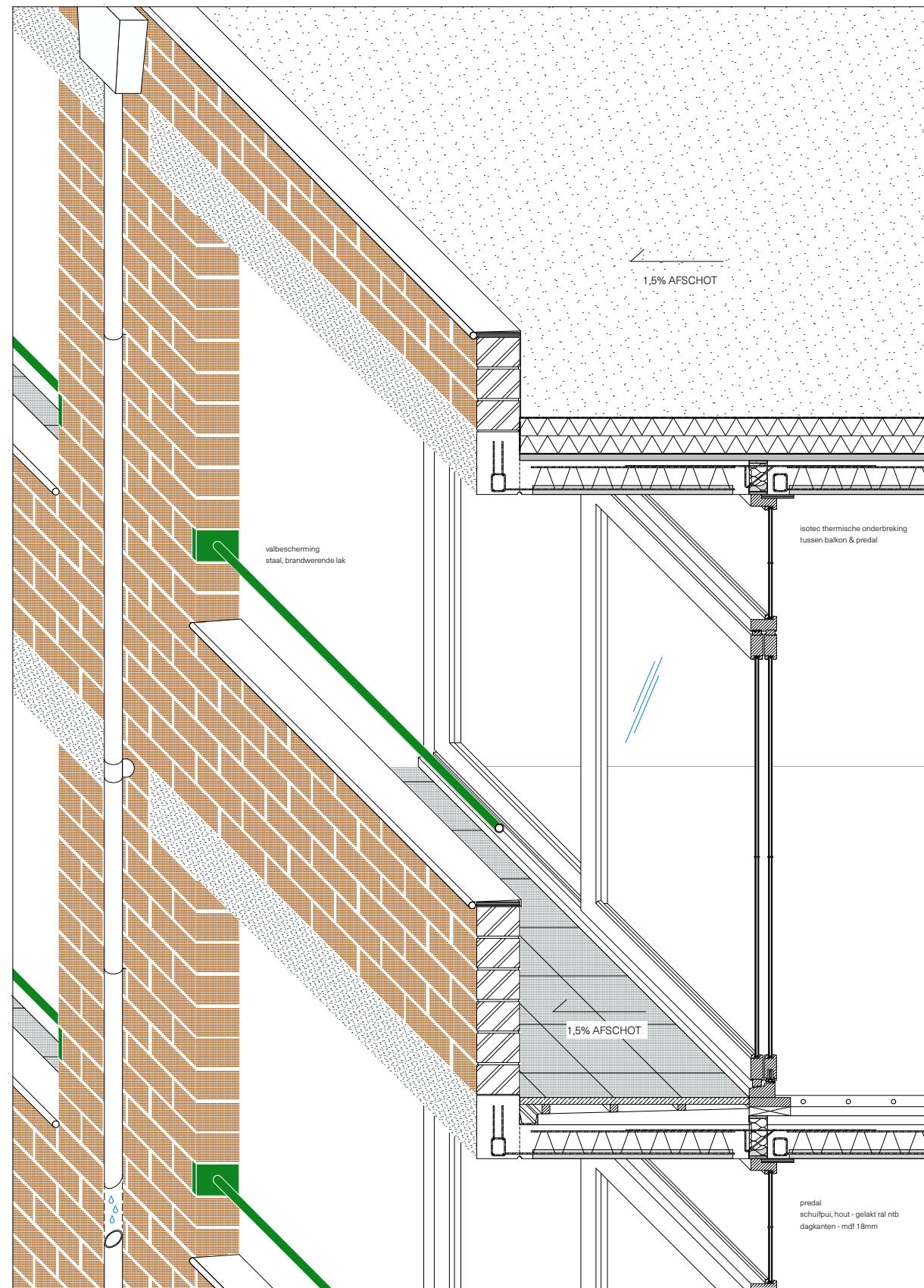
411 isometric detail loggia 1:10
