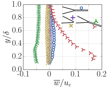
Figure 14: Spanwise mean flow component, \bar{w} .
