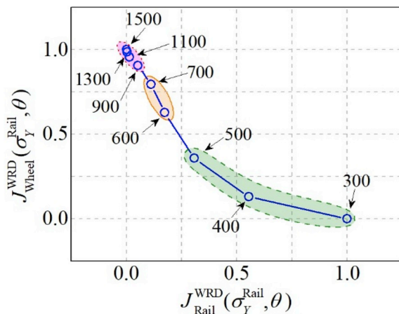
Fig. 12. Pareto front of the WRD index under the specified traffic condition. The dots and arrows indicate the values of \sigma_Y^{\text{Rail}} . 80% of the total traffics is with the wheel yield strength \sigma_Y^{\text{Wheel}} = 500 MPa, while the rest is with \sigma_Y^{\text{Wheel}} = 700 MPa.
