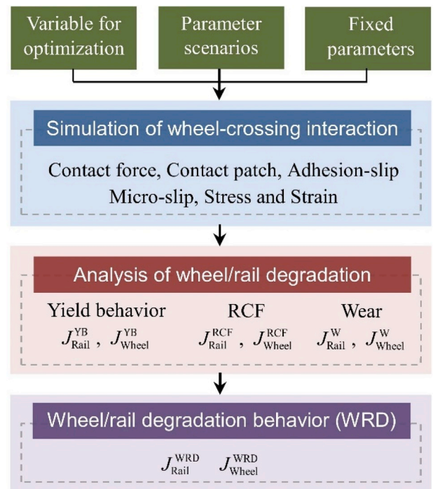
Fig. 3. Multi-criteria evaluation method for wheel/rail degradation behavior at crossings.
