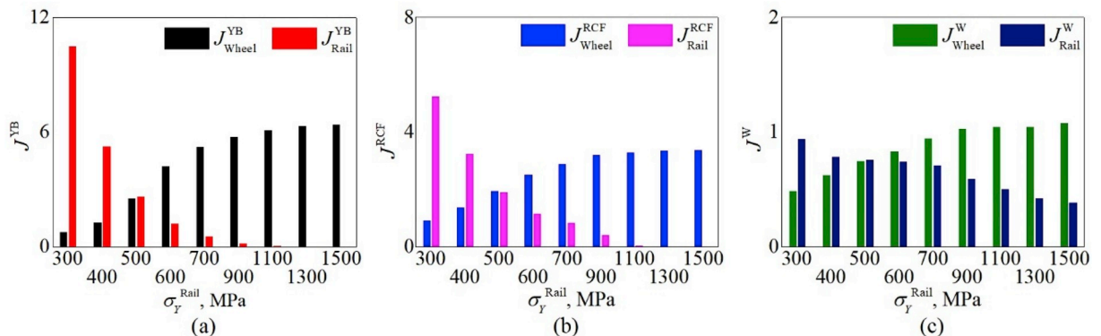
Fig. 10. Summary of wheel/rail degradation under the specified traffic condition. (a) Yield behavior, (b) RCF and (c) Wear.
