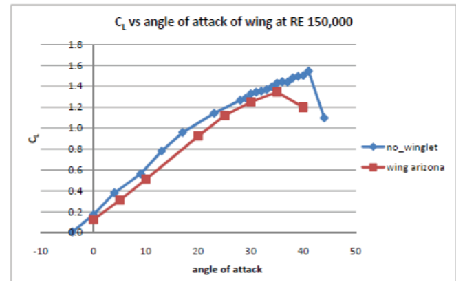
Figure 9: Comparison of CFD and Wind Tunnel Test.
