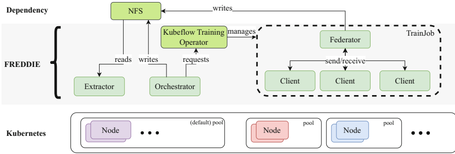
Fig. 1. Overview of Freddie . An Orchestrator and an Extractor are used for deploying experiments and collecting data. Experiments are run as TrainJobs managed by KubeFlow Training Operators. Within such a job, the defined job is run using a federator and one or more clients with local data.
