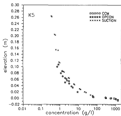
Figure 5: Time-averaged concentration profiles - test K5
