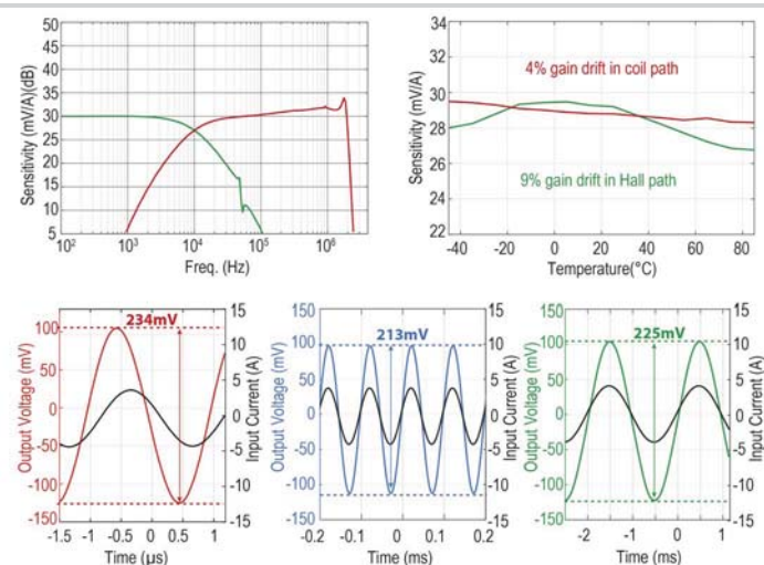
Figure 5.6.4: Measured performance of the Coil (Red) and Hall (Green) paths. Sensitivity vs. frequency (1A p-p) (top left). Sensitivity vs. temperature (1Ap-p @ 100Hz & 100kHz)(top right). Output transient response (after 1024× averaging) (8Ap-p @ 500kHz, 10kHz and 500Hz) (bottom left, middle, right).
