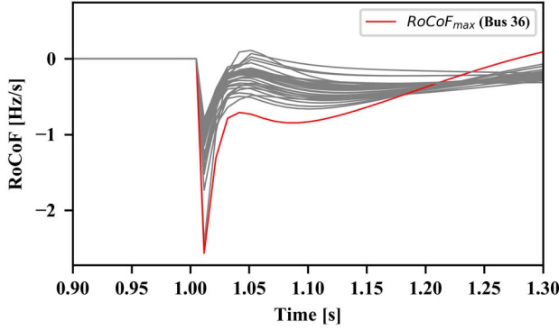
Fig. 5. RoCoF response in the 39 buses after the outage of generator G6: Case I .
