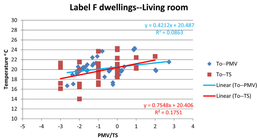
Fig. 6. Operative temperature versus PMV and RTS scatter plot and regression analysis trend line for the living rooms of F dwellings at an air speed of 0.1 m/sec.
