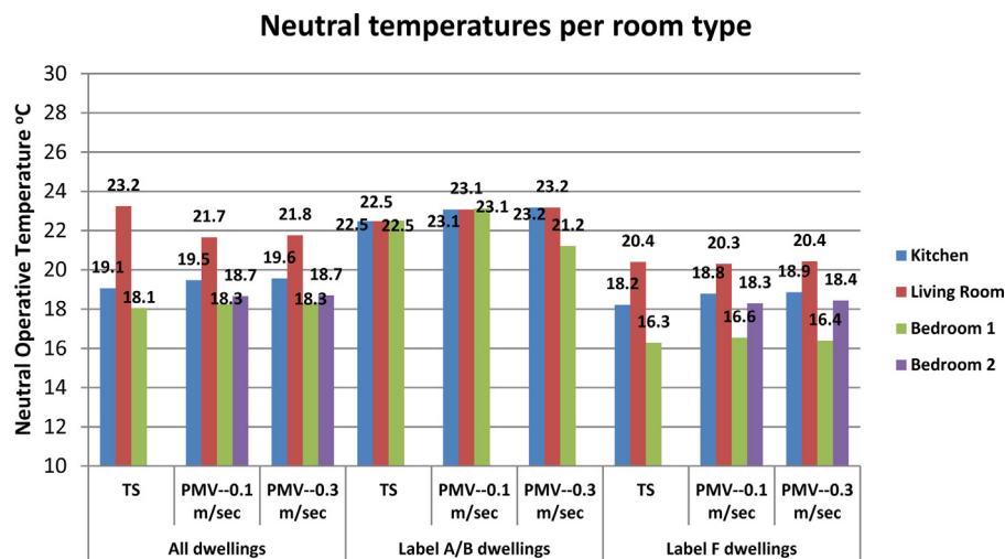
Fig. 8. Neutral operative temperatures calculated from RTS and PMV regressions for all room types and energy ratings.
