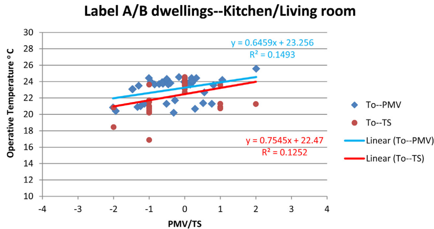
Fig. 5. Operative temperature versus PMV and RTS (reported thermal sensation) scatter plot and regression analysis trend line for the kitchen/living rooms of A/B dwellings at an air speed of 0.1 m/sec.
