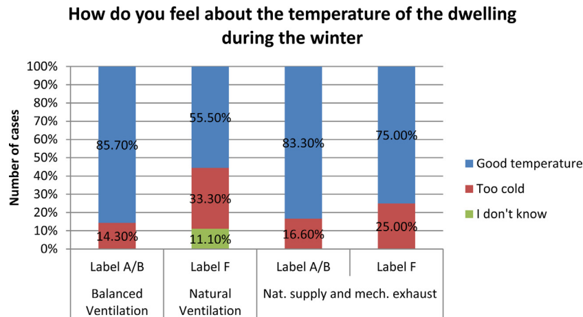
Fig. 4. Temperature perception in the winter per energy rating.
