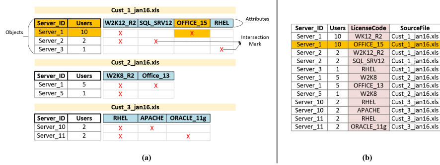
Fig. 1. An example showing related data presented in three separate spreadsheets using cross-tables in (a). (b) shows the equivalent data migrated into one relational table.
