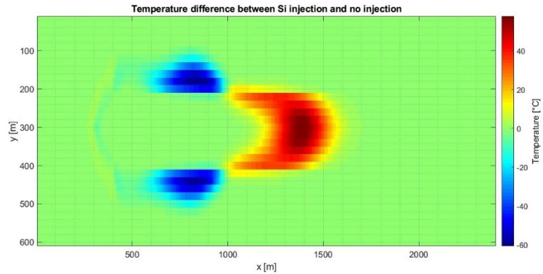
Figure 6: Temperature profiles difference. Temp. of silicate minus Temp. without silicate.
