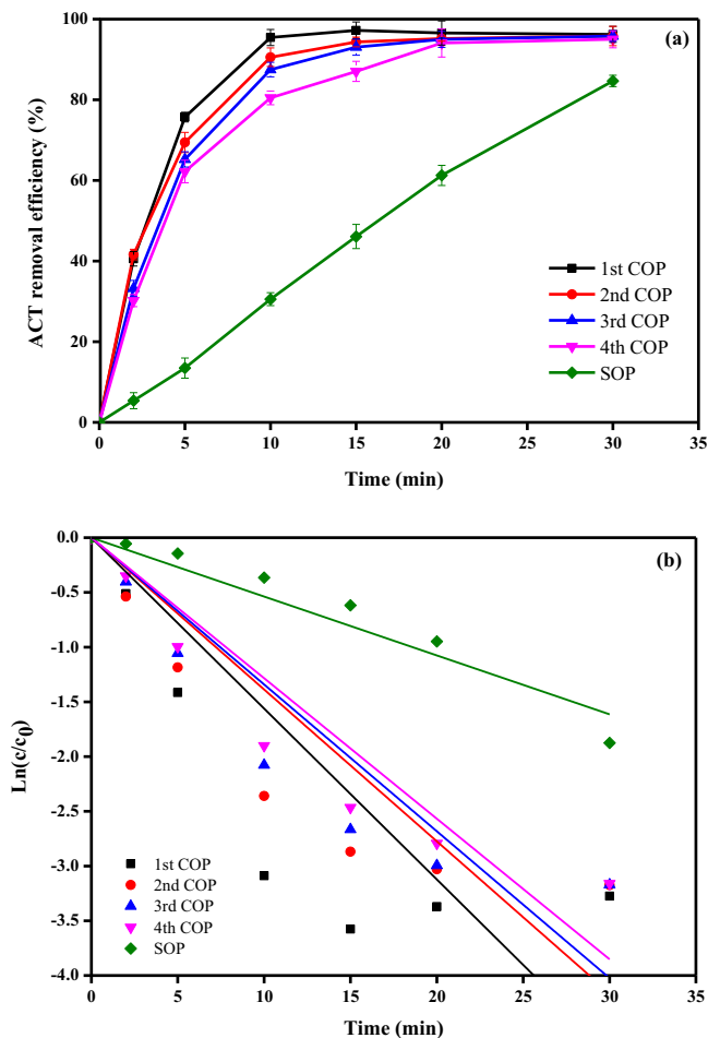
Fig. 8. The reusability of SnNaC-550 during oxidation of ACT as a function of reaction time in the COP (a) with the adjusted line equation (b) (conditions: pH: 7; ACT concentration: 50 mg/L; SnO 2 dosage: 1.3 g/L and O 3 dosage: 1.6 mg O 3 /min).
