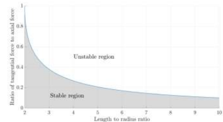
Force ratio against the length to radius ratio of a TRPT section.
