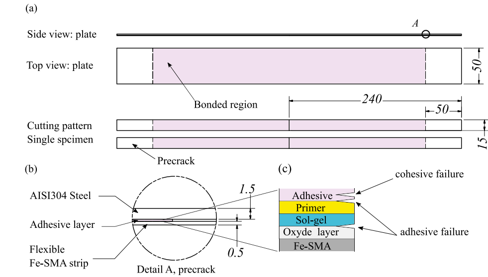
Fig. 1. Plate and specimen dimension and configuration. (a) Prepared plate and configuration of specimens cut into the plate. (b) Details of precrack and bonded plates. (c) The detailed interface between the Fe-SMA and the adhesive is the result of the surface preparation investigated. Failure location indicates the failure mode, adhesive, or cohesive.
