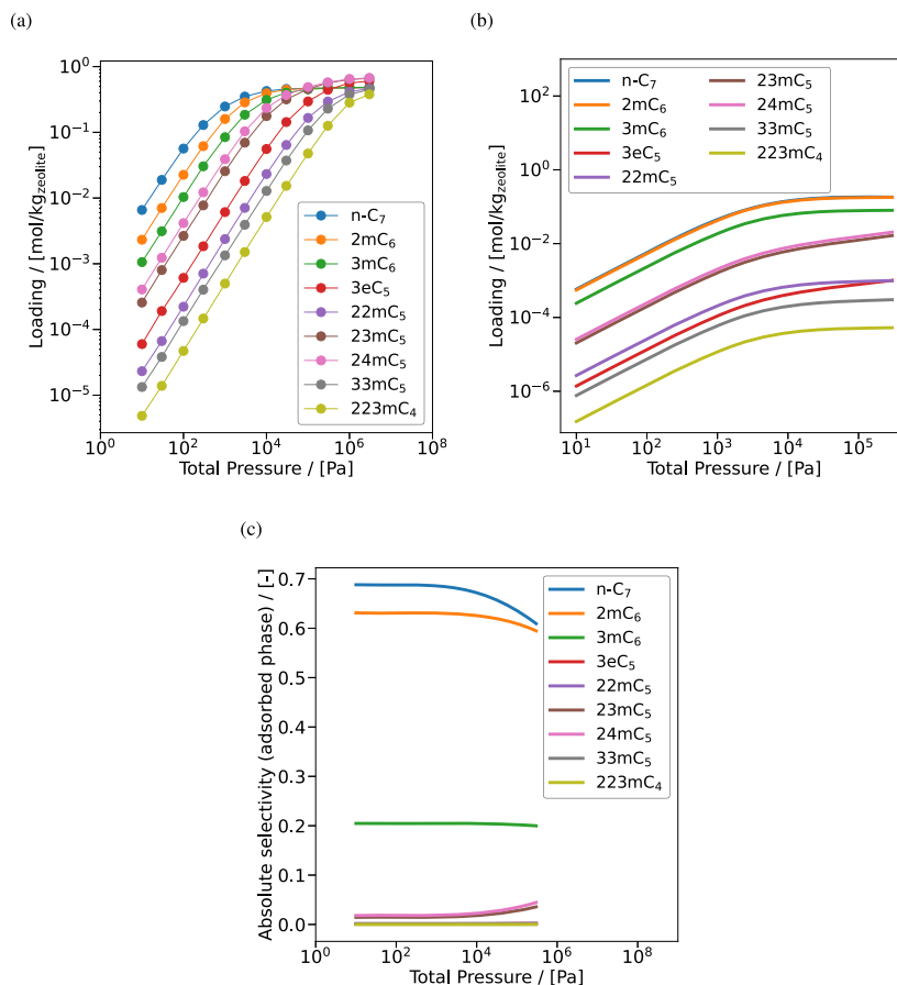
FIG. 14. (a) Pure component adsorption isotherms, (b) mixture adsorption isotherms computed using IAST, and (c) reaction equilibrium distribution (absolute selectivities) in the adsorbed phase of \text{C}_7 isomers in the MTW-type zeolite at 500 K. The pure component isotherms are fitted to single-site Langmuir-type isotherms.
