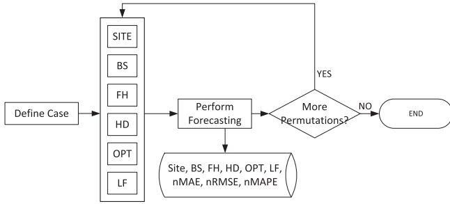
Fig. 4. Implemented simulation approach for Step 2.
