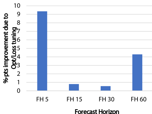
Fig. 14. Additional improvement in nMAE as a result of optimizer-loss function tuning.
