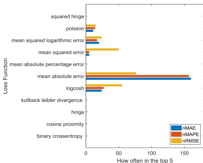
Fig. 11. Ranking of loss functions.
