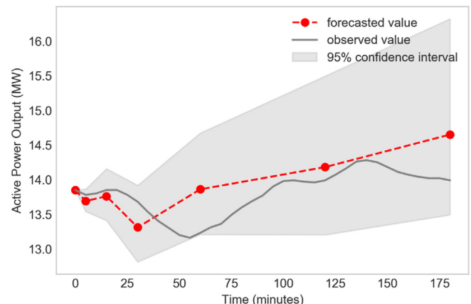
Fig. 15. Observed versus forecasted values of most accurate implemented algorithm.
