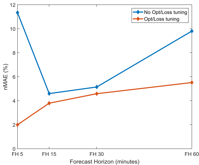
Fig. 13. nMAE comparison with and without optimizer-loss function tuning.
