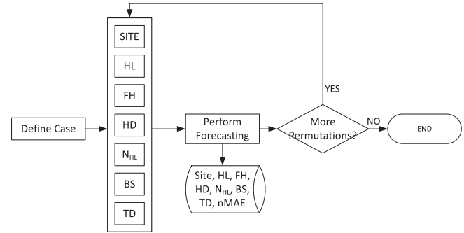
Fig. 3. Implemented simulation approach for Step 1.
