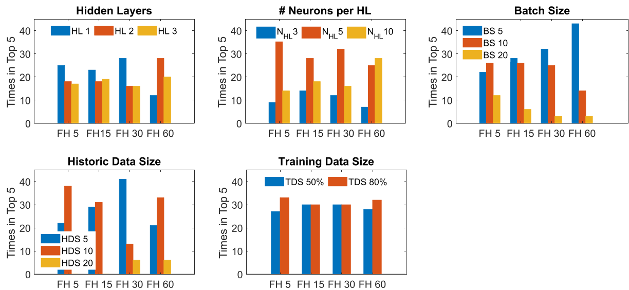
Fig. 8. Parametric evaluation of ANN based forecast model.
