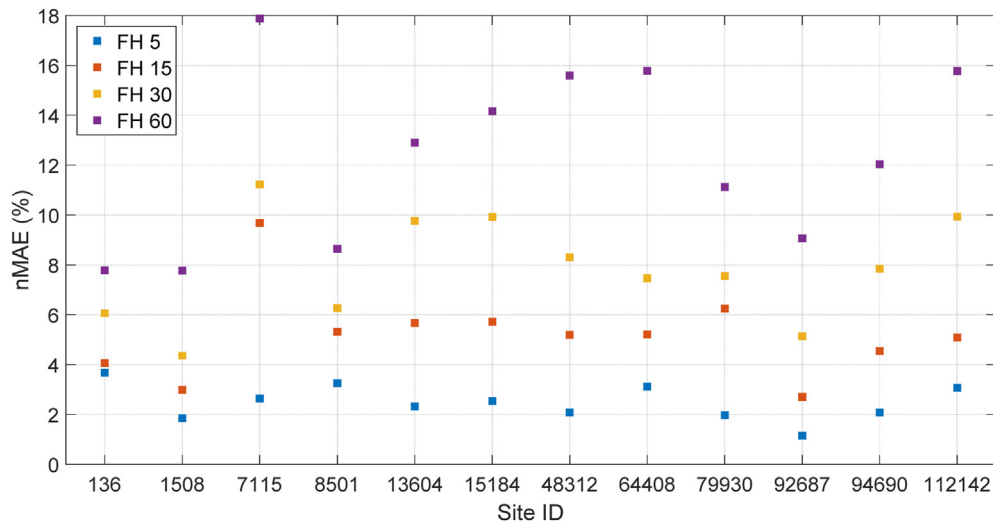
Fig. 7. First Quartile of nMAE for 12 wind farms across four forecast horizons.
