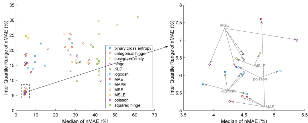
Fig. 12. Median versus Inter Quartile Range for loss functions.
