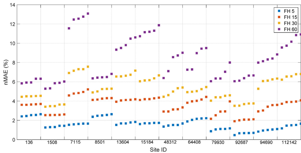
Fig. 6. nMAE for 12 wind farms across four forecast horizons.
