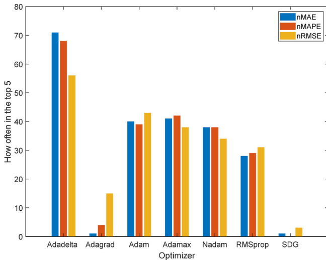
Fig. 9. Ranking of optimizers.
