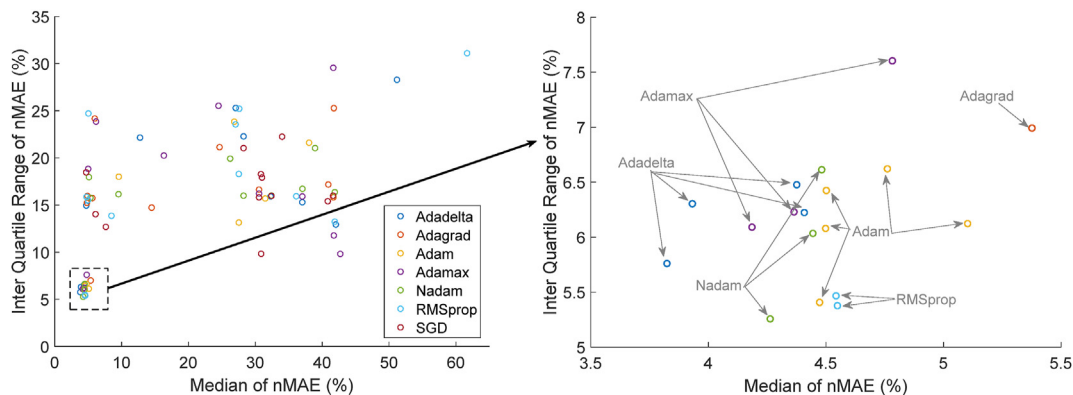
Fig. 10. Median versus Inter Quartile Range for optimizers.
