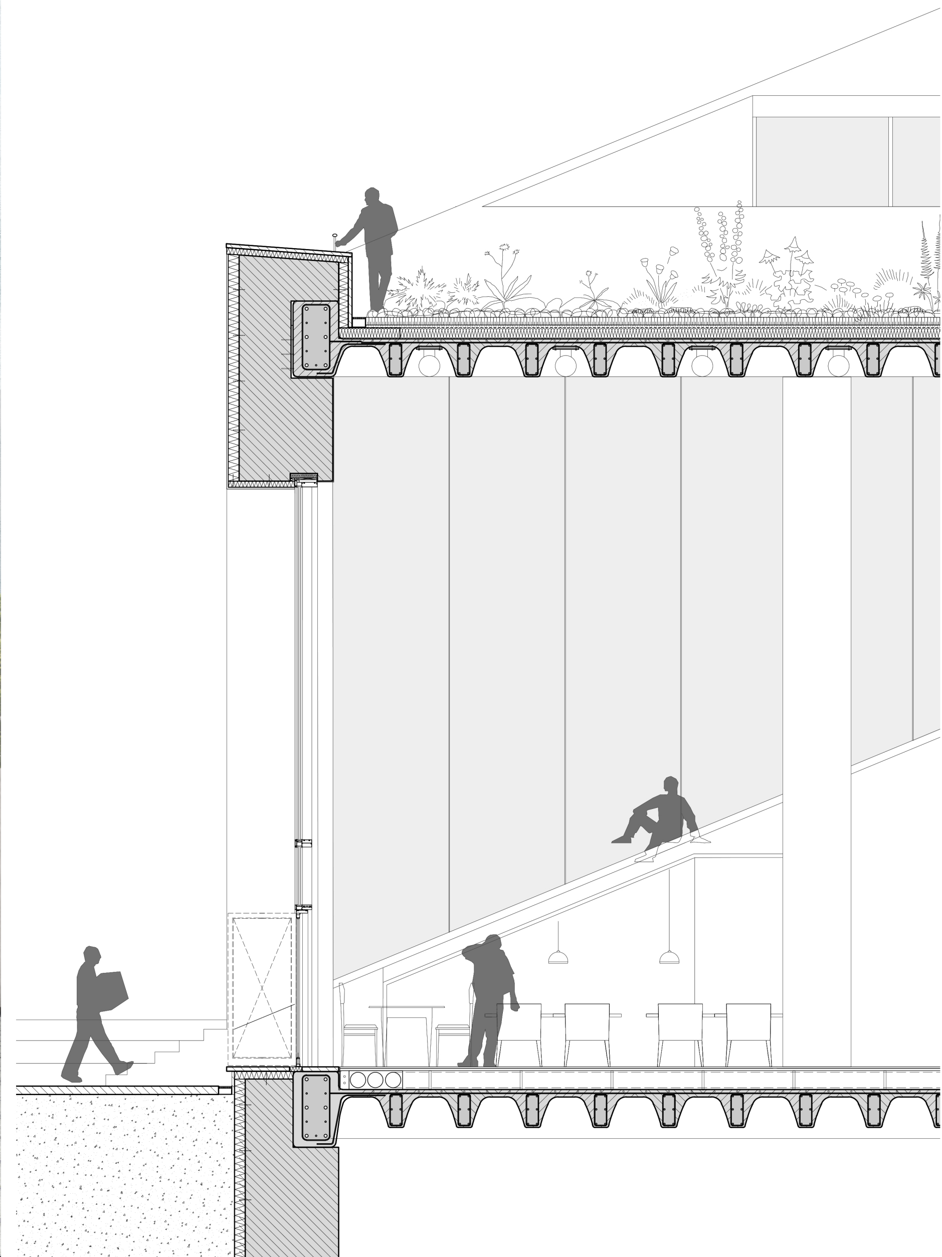
DETAIL FACADE
