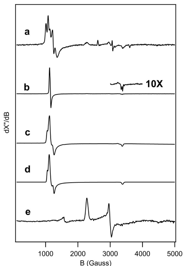
Fig. 4 EPR spectra of AoCld without and with several ligands. a AoCld 75 \mu M monomer concentration in 100 mM KPi pH 7.0. b AoCld-fluoride adduct in 100 mM KPi pH 7.0 containing 250 mM NaF showing the ^{19}\text{F} hyperfine splitting. c AoCld-acetate adduct in 100 mM acetate pH 5.0 experimental spectrum and d simulation of the AoCld-acetate spectrum. Simulation parameters: two components: main component 71% g_{z,y,x}=5.98, 5.70, 1.985 ; W_{zyx}=2.7, 6.0, 3.0 mT; minor component 29% g_{z,y,x}=6.36, 5.38, 1.985 ; W_{zyx}=1.5, 2.0, 3.0 mT. e AoCld-Imidazole adduct in 100 mM KPi pH 7.0 containing 1 mM imidazole. EPR conditions: Microwave frequency, 9.405 GHz; Microwave power, 20 mW; Modulation frequency, 100 kHz; Modulation amplitude, 1.0 mT; Temperature, 20 K. The spectra were normalized for the maximal signal amplitude
