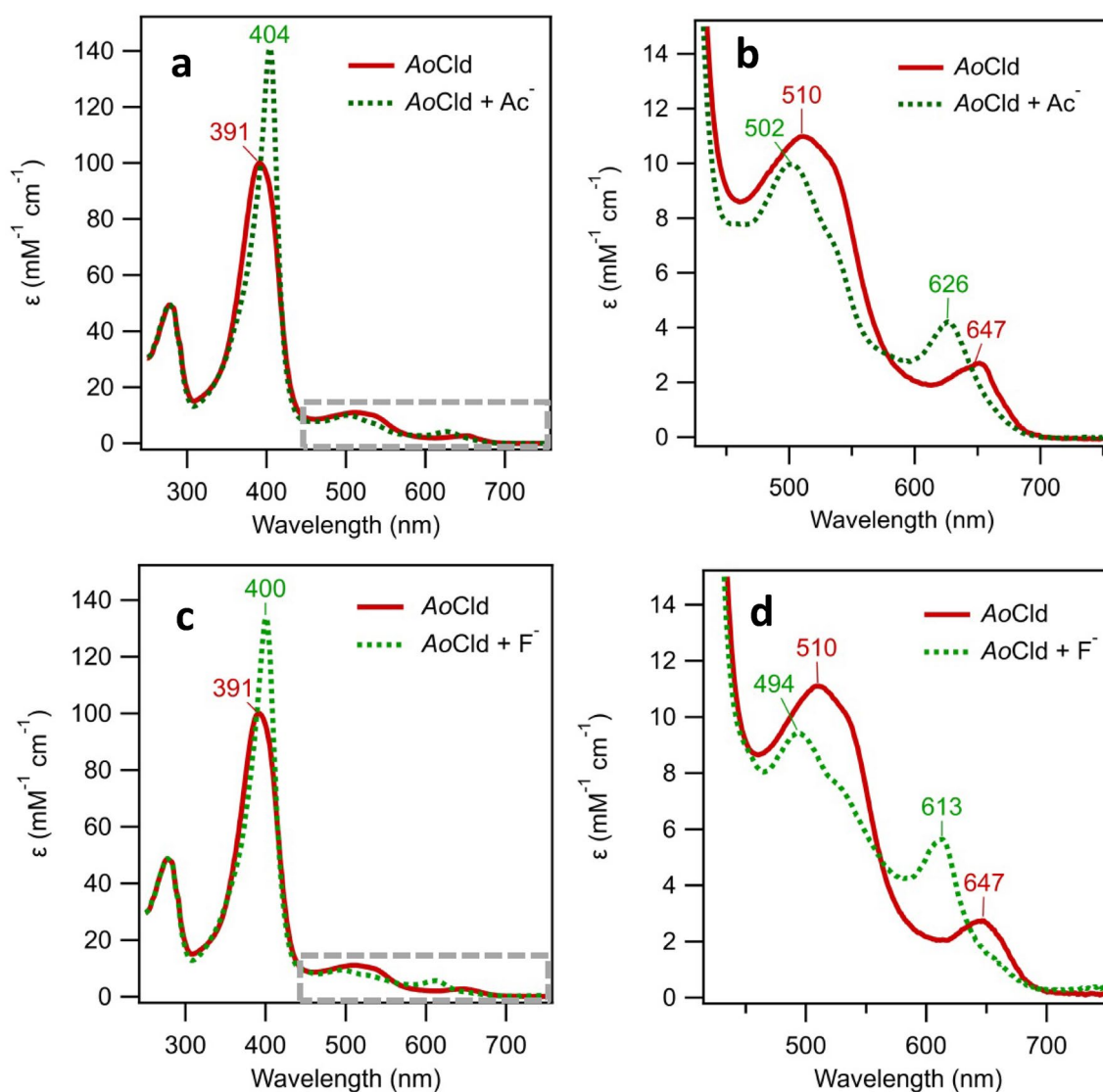
Fig. 3 UV-visible spectra of AoCld-acetate and fluoride adducts. 10 \mu\text{M} AoCld solutions were recorded in 1 mL quartz cuvette with 1.0 cm path length. a , b AoCld (red solid line) and AoCld-acetate adduct (green dotted line); c , d AoCld (red solid line) and AoCld-flu-
