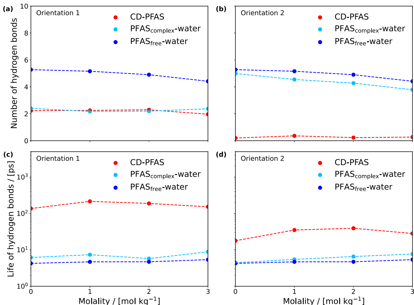
Figure 10. Number (a, b) and lifetime (c, d) of hydrogen bonds in \beta -CD-PFOA inclusion complexes under different NaCl molalities for Orientation 1 (a, c) and Orientation 2 (b, d). PFAS complex denotes PFOA in the inclusion complex and PFAS free denotes free PFOA in pure aqueous solution.
