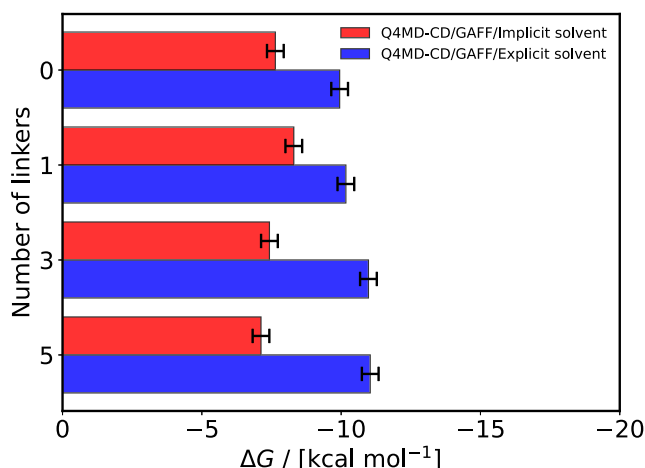
Figure 13. Host-guest binding free energies in \beta -CD and PFOA systems with different numbers of phenyl linkers. The apparent free energies are used here (eq 1).
