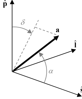
Figure 2 Definition of cone, \alpha , and clock, \delta , angles of the solar sail acceleration vector in S(\hat{\mathbf{s}}, \hat{\mathbf{l}}, \hat{\mathbf{p}}) reference frame.
