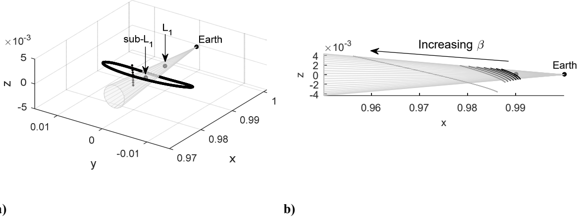
Figure 8 Solar sail halo orbits fitting around a 5 deg solar exclusion zone. a) \beta = 0.0363 with dots indicating initial conditions of family of solar sail halo orbits for \beta = 0.0363 . b) (x,z)-view for \beta = 0.01 - 0.04 and 0.08.
