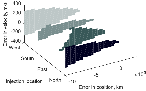
Figure 21 Recoverable injection error for different injection locations along solar sail halo orbit with \beta_{nom} = 0.0363 . a) FPF sail. b-d) Heliogyro with (b) \beta_{max} = 0.03732 , (c) \beta_{max} = 0.038 , and (d) \beta_{max} = 0.04 .
