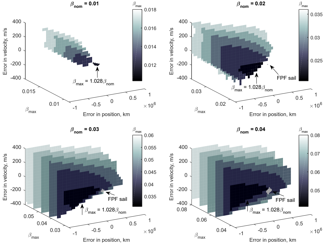
Figure 19 Orbital control of solar sail halo orbits with \beta_{nom} = 0.01, 0.02, 0.03 , and 0.04 . Recoverable injection error for FPF sail (only visible for \beta_{nom} = 0.02, 0.03 , and 0.04 ) and heliogyro for different values for \beta_{max} .
