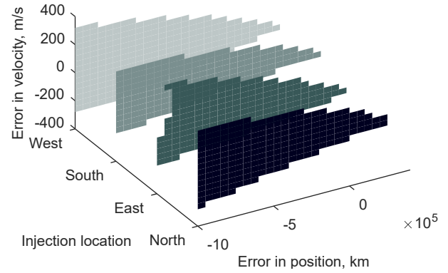
Figure 21 Recoverable injection error for different injection locations along solar sail halo orbit with \beta_{nom} = 0.0363 . a) FPF sail. b-d) Heliogyro with (b) \beta_{max} = 0.03732 , (c) \beta_{max} = 0.038 , and (d) \beta_{max} = 0.04 .
