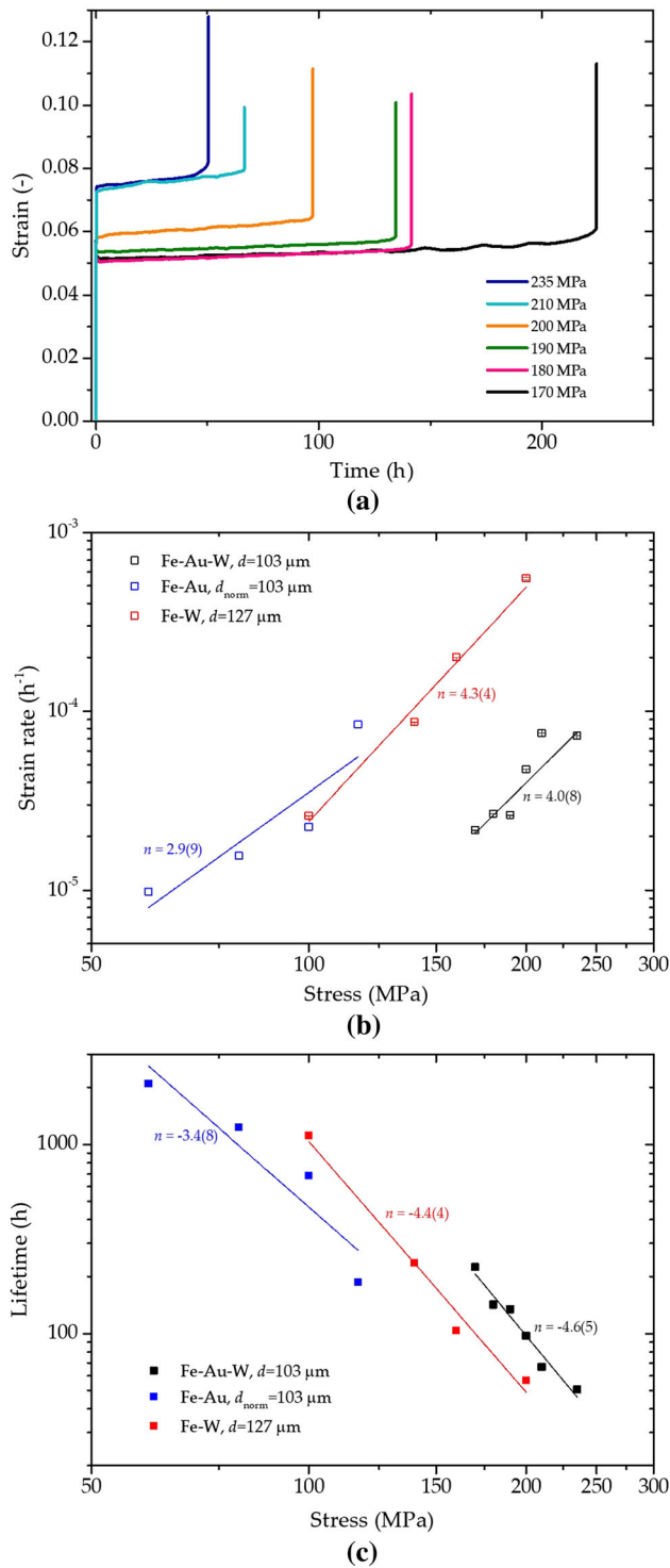
Fig. 1—(a) Creep curves for the Fe-Au-W alloy samples with different constant stress levels at a temperature of 823 K (550 °C). (b) Derived steady-state strain rate and (c) creep lifetime as a function of applied stress. The strain rates and lifetimes of the previous Fe-Au [19,20] and Fe-W [18] samples are also summarized and compared in (b) and (c).
