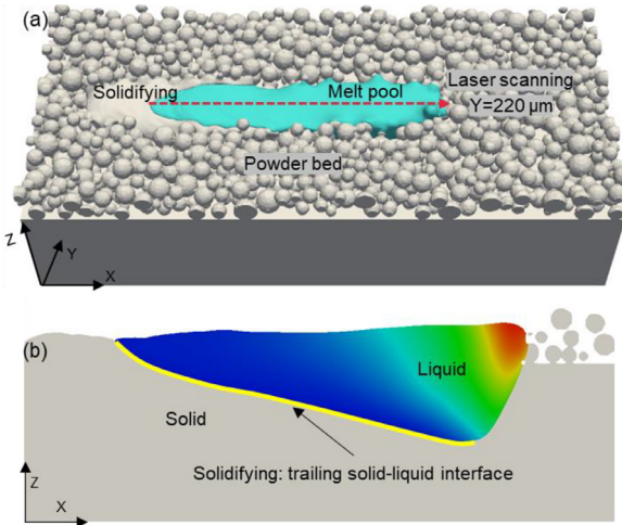
Fig. 2. (a) Melting and solidifying process and (b) schematic diagram of the solidification interface, indicated by the yellow line, for computing the solidification rate and thermal gradient.
