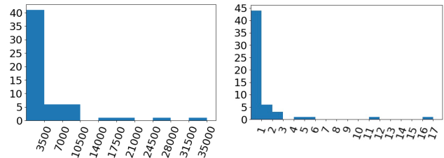
(a) Code density of logging. (b) Logging code churn rate (%).
