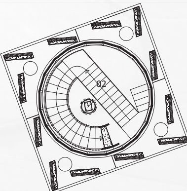
1:50 Plan Ground Level
