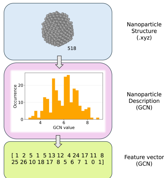
Fig. 1 Top) a snapshot of one Pt nanocatalyst of 518 atoms. Mid) its GCN distribution. Bottom) the associated feature vector used as input in the ML workflow.
