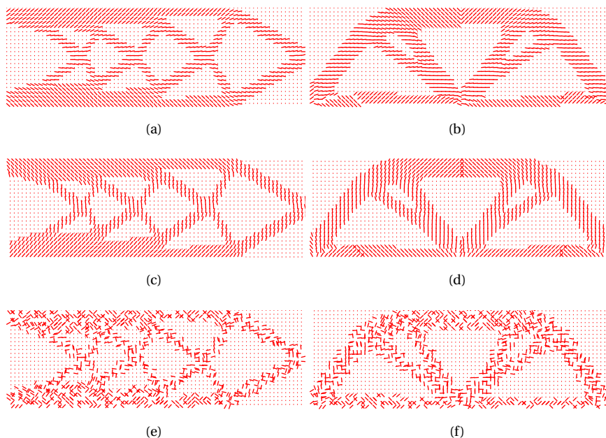
Figure B.1: Effect of initial state on optimized design layout and optimized deposition directions: (a), (c) and (e) provide optimized design layouts and optimized deposition directions with initial states as 0^\circ , 90^\circ and completely random for the cantilever problem. (b), (d) and (f) show optimized design layouts and optimized deposition directions with initial states as 0^\circ , 90^\circ and completely random for the bridge problem.
