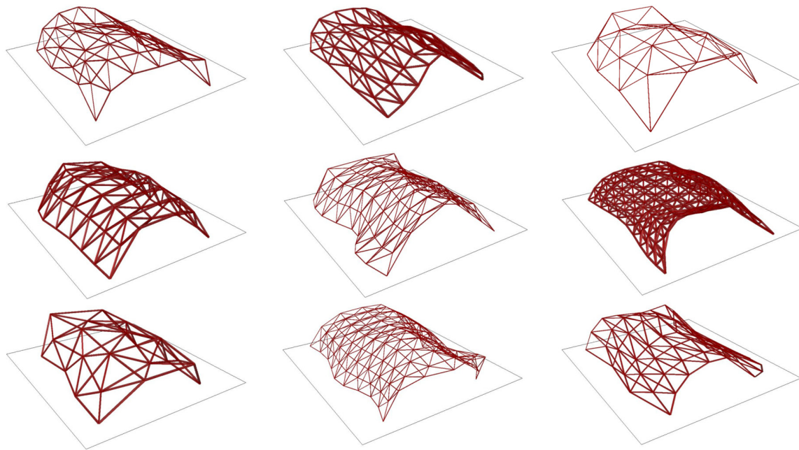
Figure 12. Some alternatives of the design problem.
