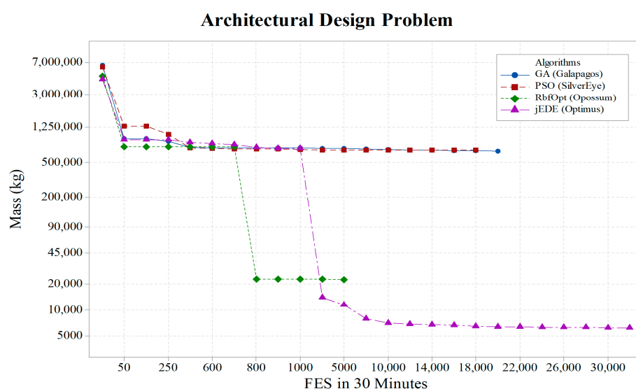
Figure 13. Convergence graph of architectural design problem.
