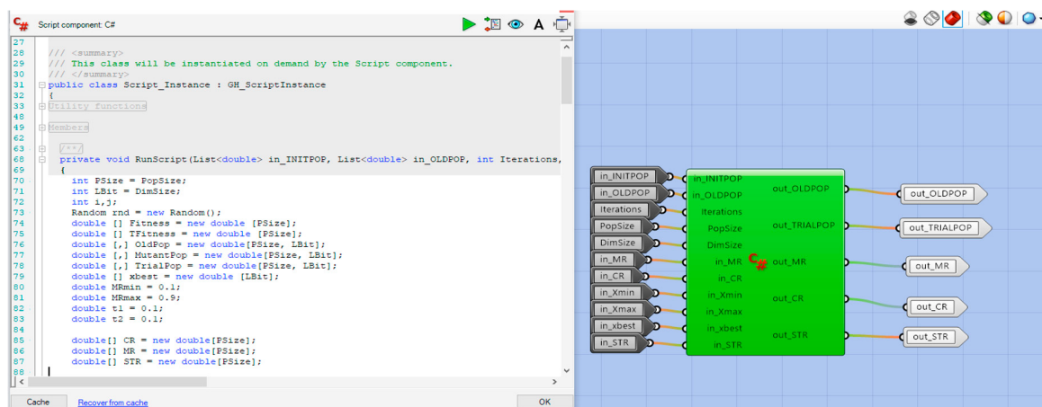
Figure 5. Example cluster implementation for self-adaptive differential evolution algorithm with ensemble of mutation strategies (jeDE) component.
