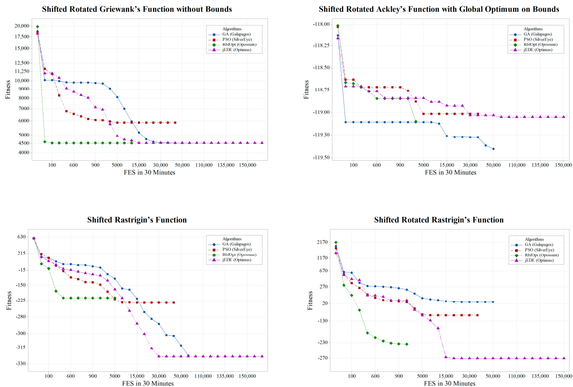
Figure 9. Convergence graphs of CEC2005 benchmark functions.
