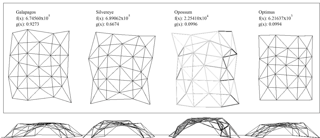
Figure 14. Optimized results of design problem.
