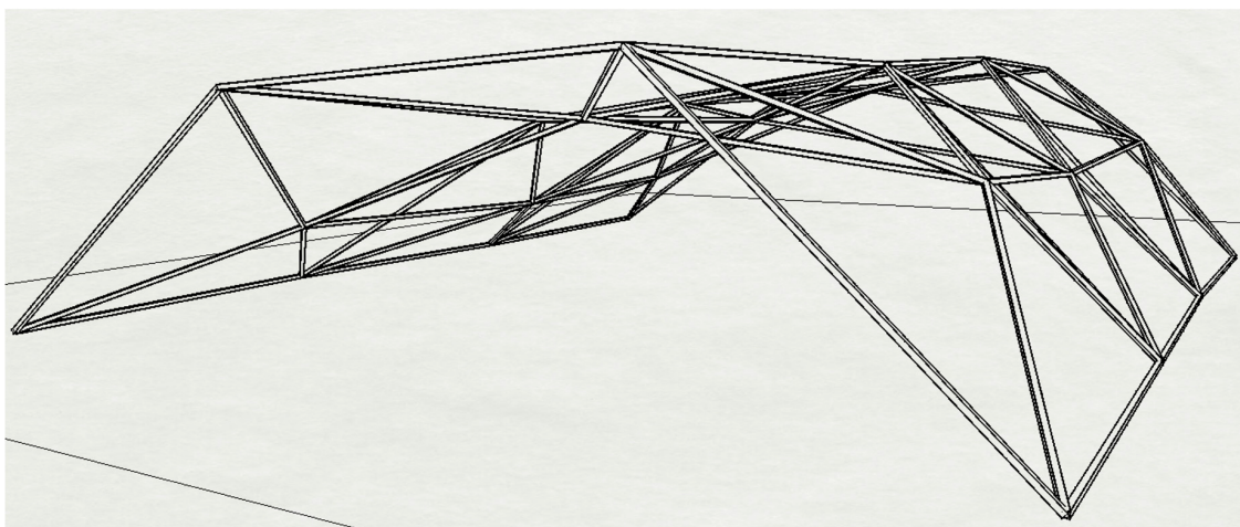
Figure 15. Illustration of the best alternative (Optimus) result for design optimization problem.
