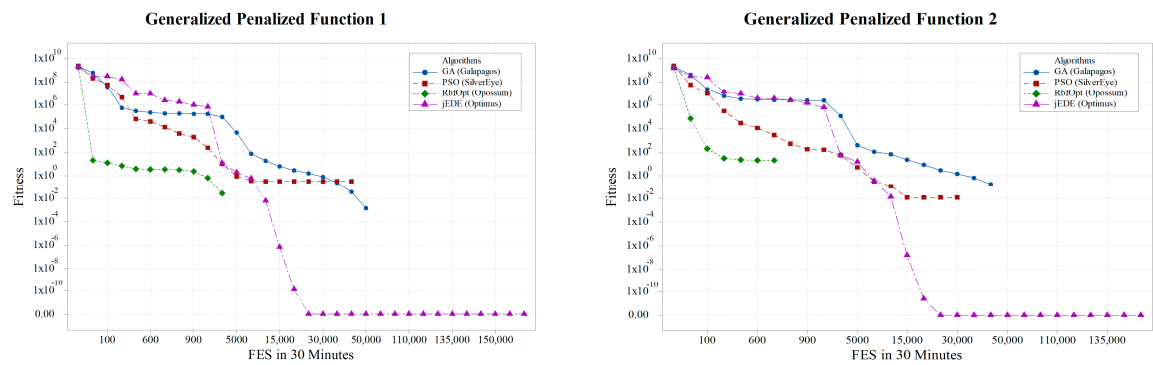
Figure 8. Convergence graphs of standard benchmark functions.
