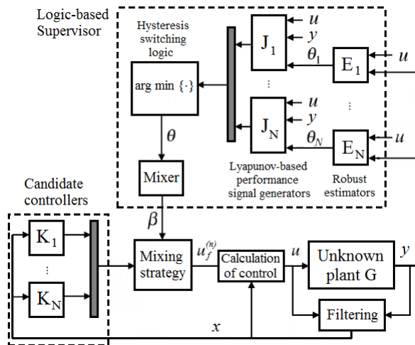
Fig. 1. Lyap-AMC architecture
