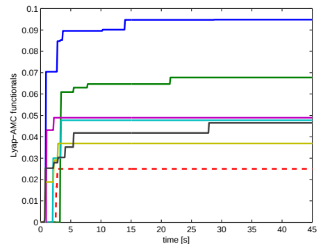
Fig. 7. k^* = 0.2 : Performance signals for Lyap-AMC: in a dashed line the signal \mathcal{J}_3 associated with the desired controller is shown
