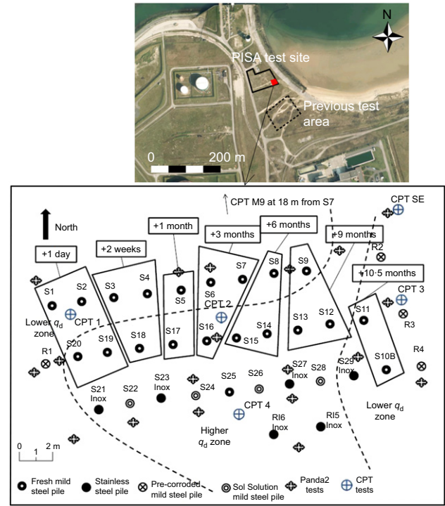
Fig. 6. Dunkirk site layout
