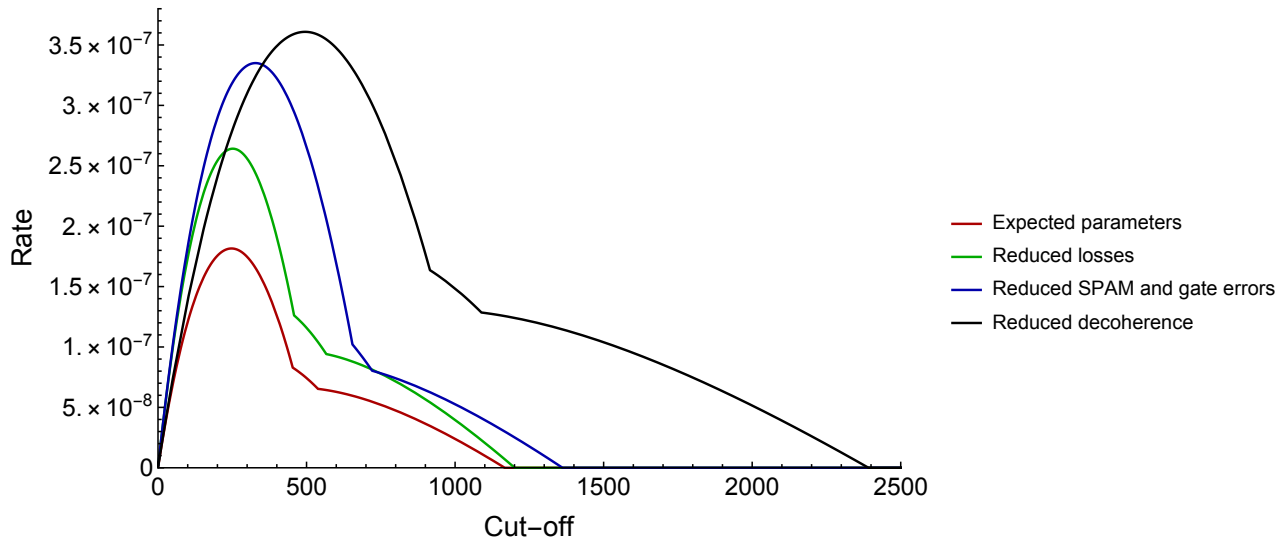
FIG. 5. Secret-key rate as a function of the cut-off for the expected parameters with the repeater positioned half-way between Alice and Bob. The reduced losses are for p'_{\text{app}} = (p_{\text{app}})^{0.9} and p'_{\text{ps}} = (p_{\text{ps}})^{0.9} , the reduced SPAM (state preparation and measurement) and gate errors are for F'_{\text{gm}} = (F_{\text{gm}})^{0.7} and F'_{\text{prep}} = (F_{\text{prep}})^{0.7} and the reduced decoherence is for a' = a/2 and b' = b/2 . The optimal n^* shifts depending on the parameters. The kinks arise due to the fact that we optimise over two protocols: fully asymmetric BB84 and symmetric six-state protocol with advantage distillation which itself consists of two subprotocols. The optimal protocol depends on the bit error rates. The data have been plotted for the distance of 15L_0 , where L_0 = 0.542 km.
