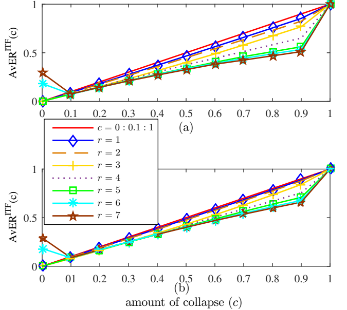
Fig. 10. Reverberant environment (office): Average ITF error ratio as a function of c for 1 \leq r \leq 7 for (a) k_{\max} = 10 and (b) k_{\max} = 50 . The solid line is the c values.
