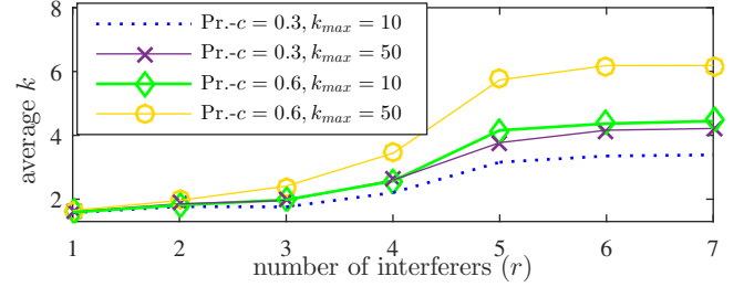
Fig. 6. Anechoic environment: Average number of iterations as a function of simultaneously present interferers, r .
