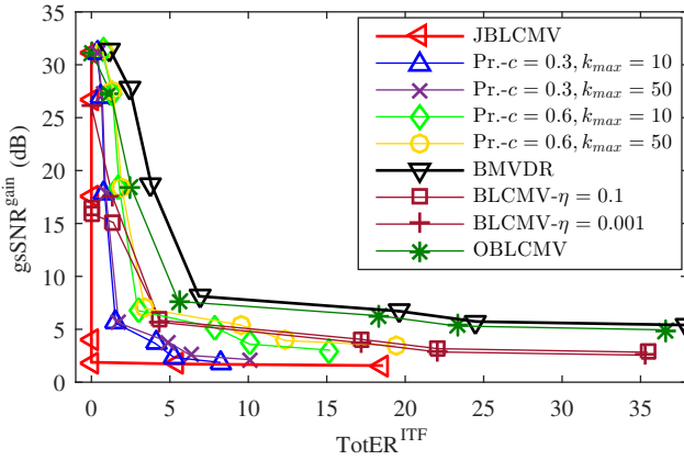
Fig. 9. Reverberant environment (office): Combination of performance curves from Fig. 8 for the competing methods in terms of (a) noise reduction, (b) ITF error for different number of simultaneously present interferers r . The counting of r starts at the top left part of each curve.
