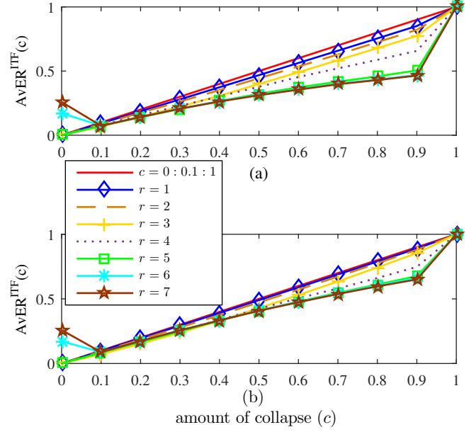
Fig. 5. Anechoic environment: Average ITF error ratio as a function of c for 1 \leq r \leq 7 for (a) k_{\max} = 10 and (b) k_{\max} = 50 . The solid line is the c values.
