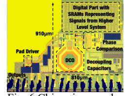
Fig. 6 Chip micrograph.
